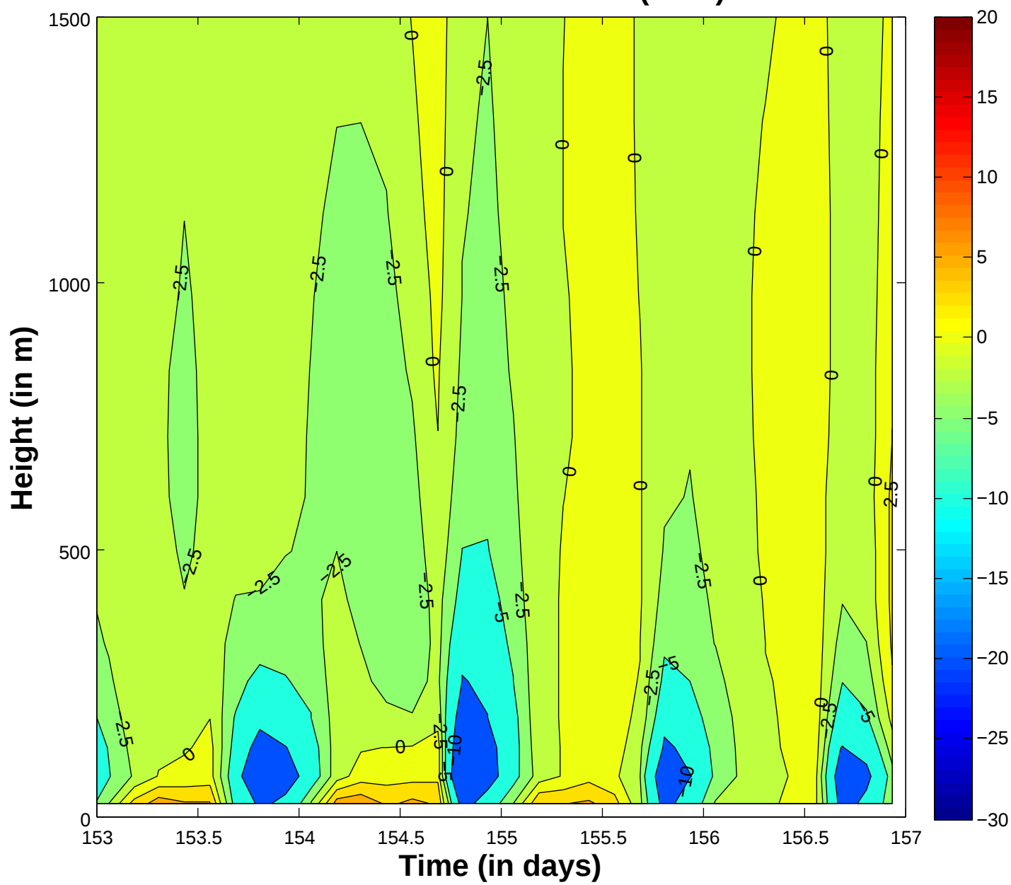
Run 304 – 204 Total TKE ( \text{m}^2/\text{s}^2 )
