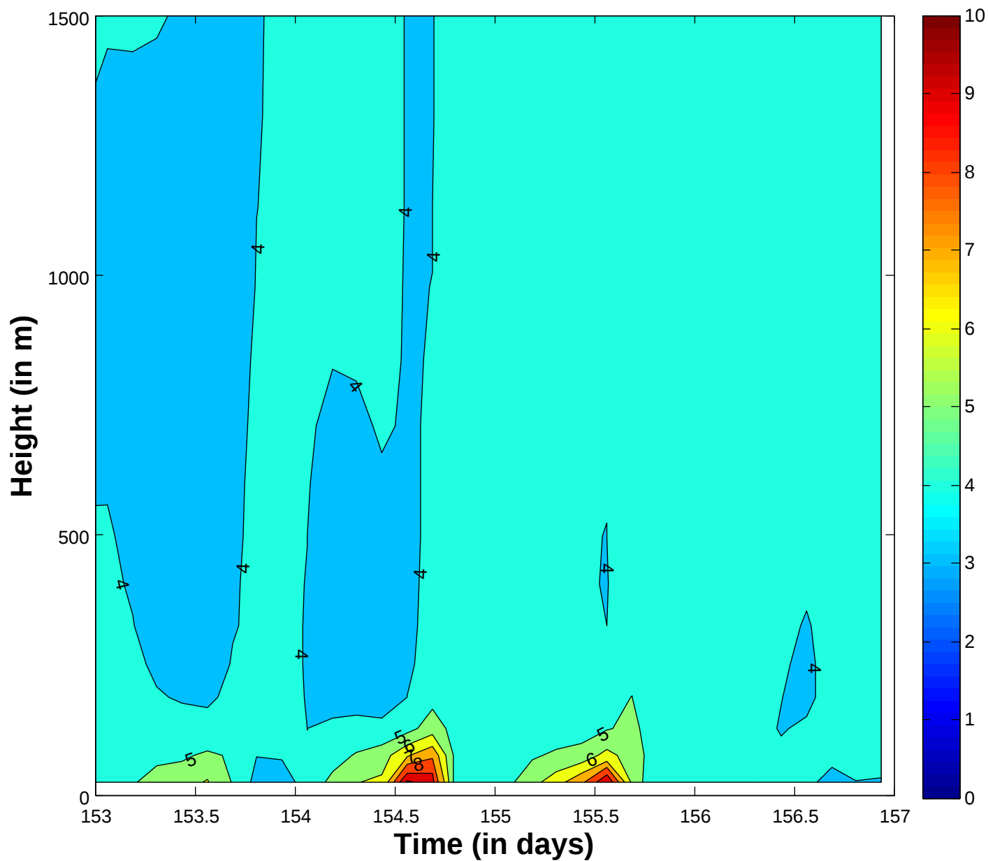
Run 306 – 206 \theta
