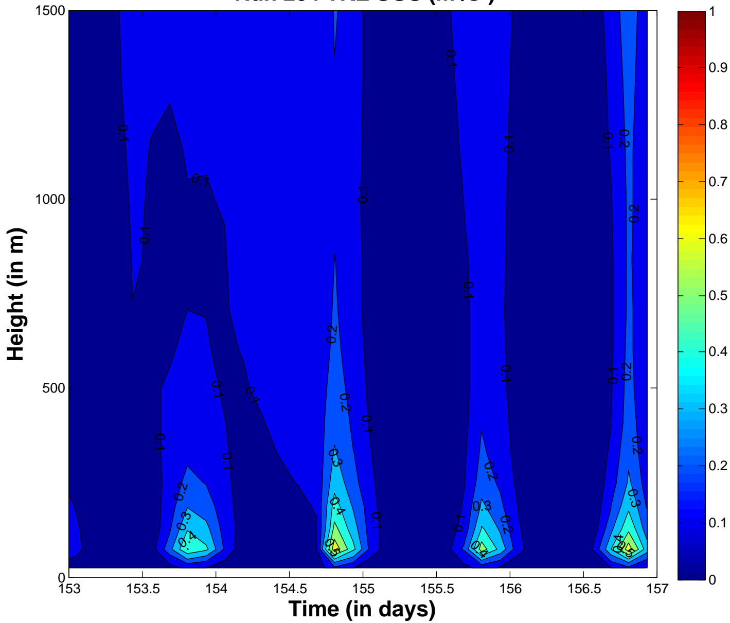
Run 204 TKE SGS ( \text{m}^2/\text{s}^2 )
