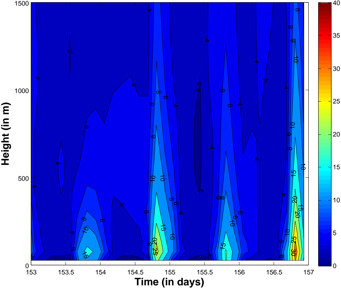
Run 206 TKE Resolved ( \text{m}^2/\text{s}^2 )
