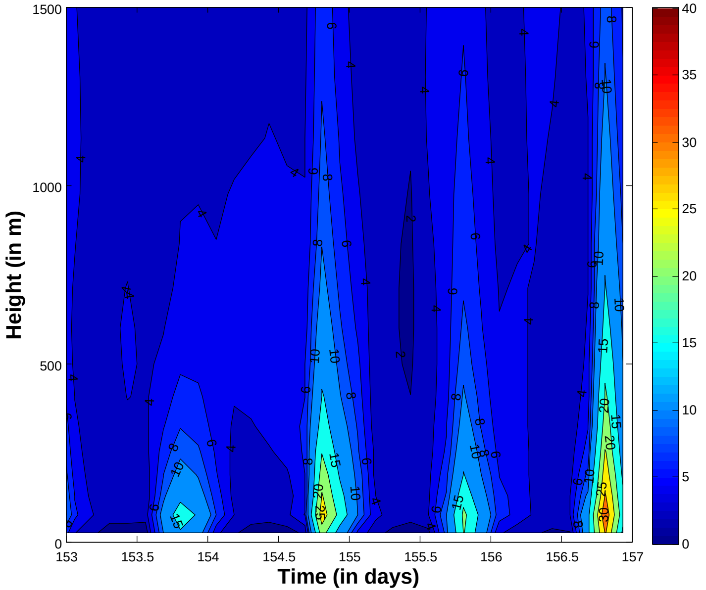
Run 206 Total TKE ( \text{m}^2/\text{s}^2 )
