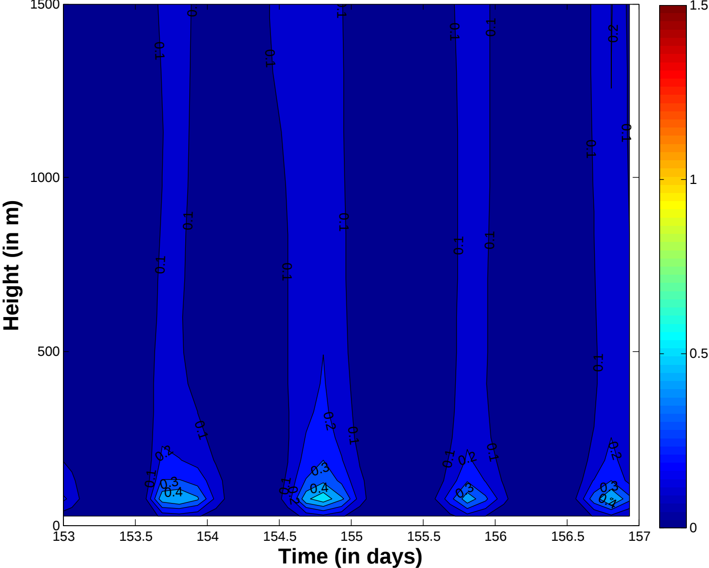
Run 208a TKE SGS ( \text{m}^2/\text{s}^2 )
