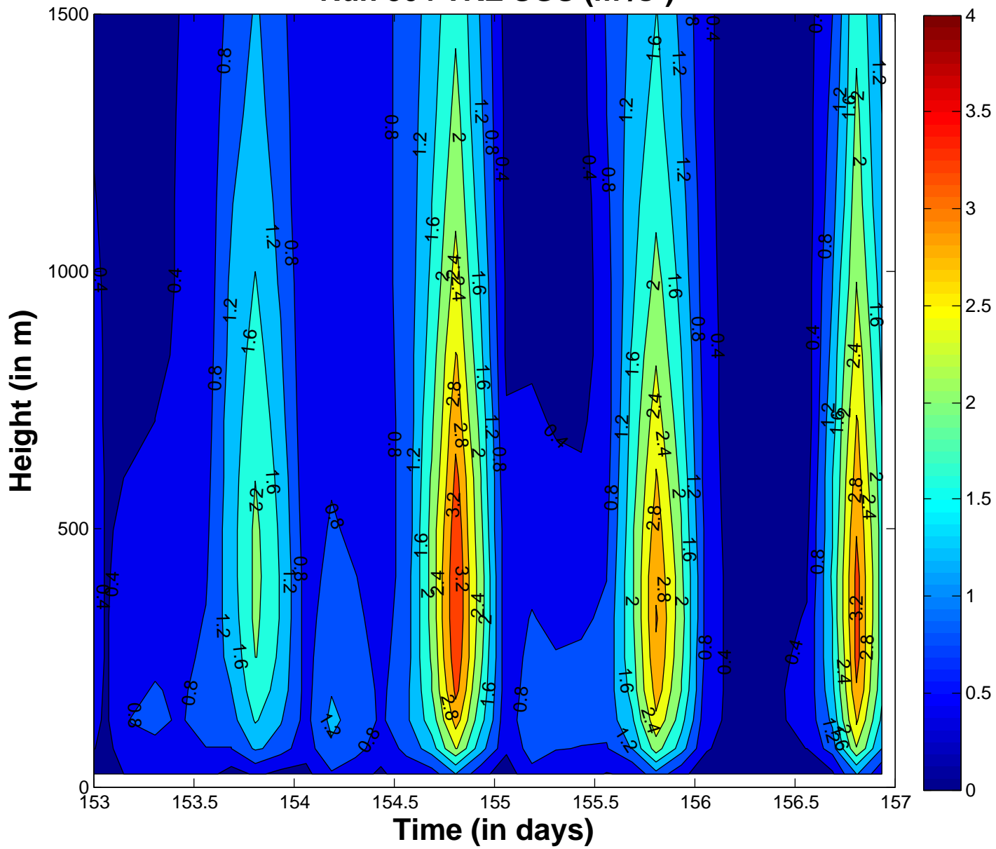
Run 304 TKE SGS ( \text{m}^2/\text{s}^2 )
