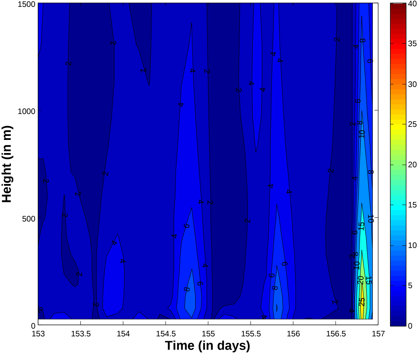
Run 306 TKE Resolved ( \text{m}^2/\text{s}^2 )
