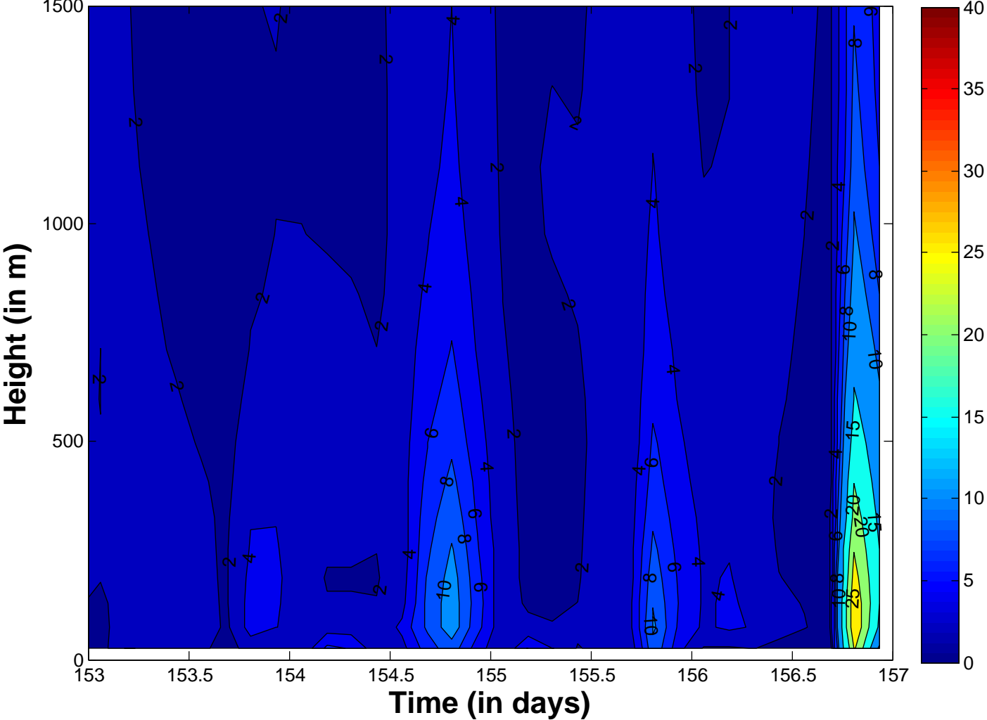
Run 308a TKE Resolved ( \text{m}^2/\text{s}^2 )
