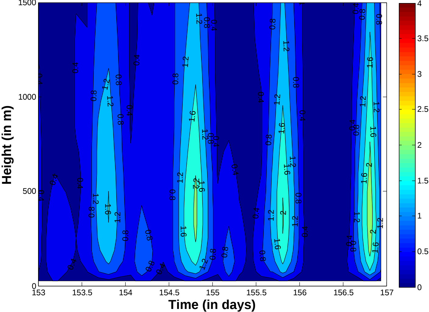
Run 308a TKE SGS ( \text{m}^2/\text{s}^2 )
