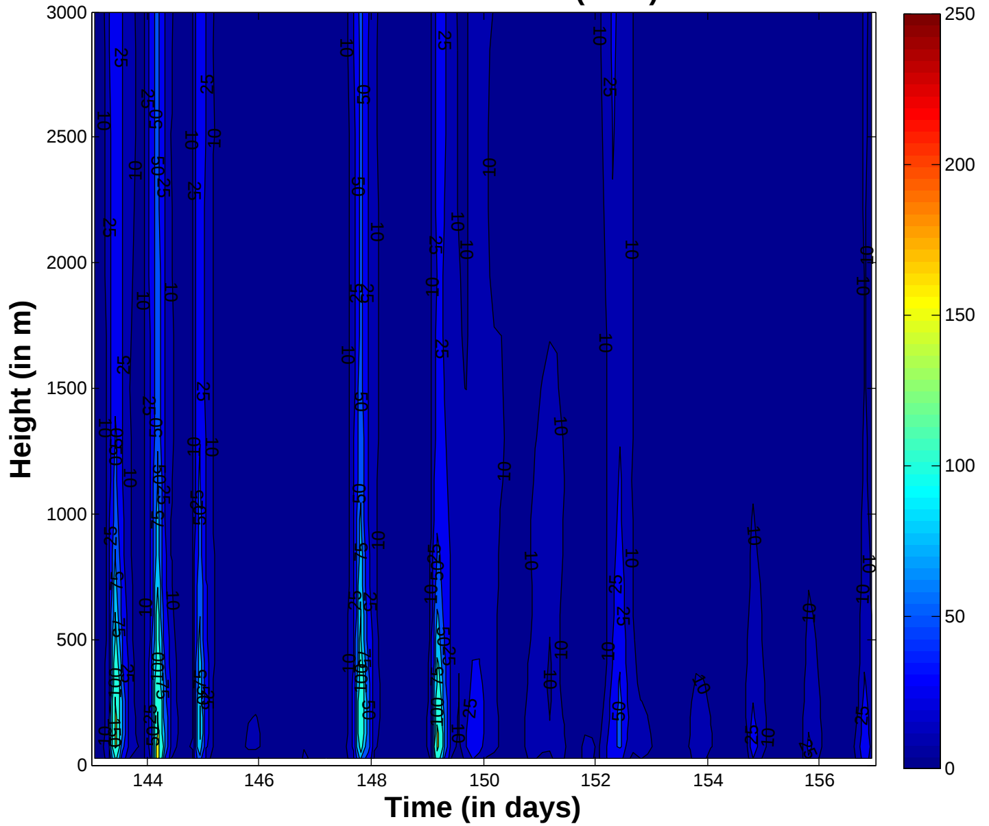
Run 204 Total TKE ( \text{m}^2/\text{s}^2 )
