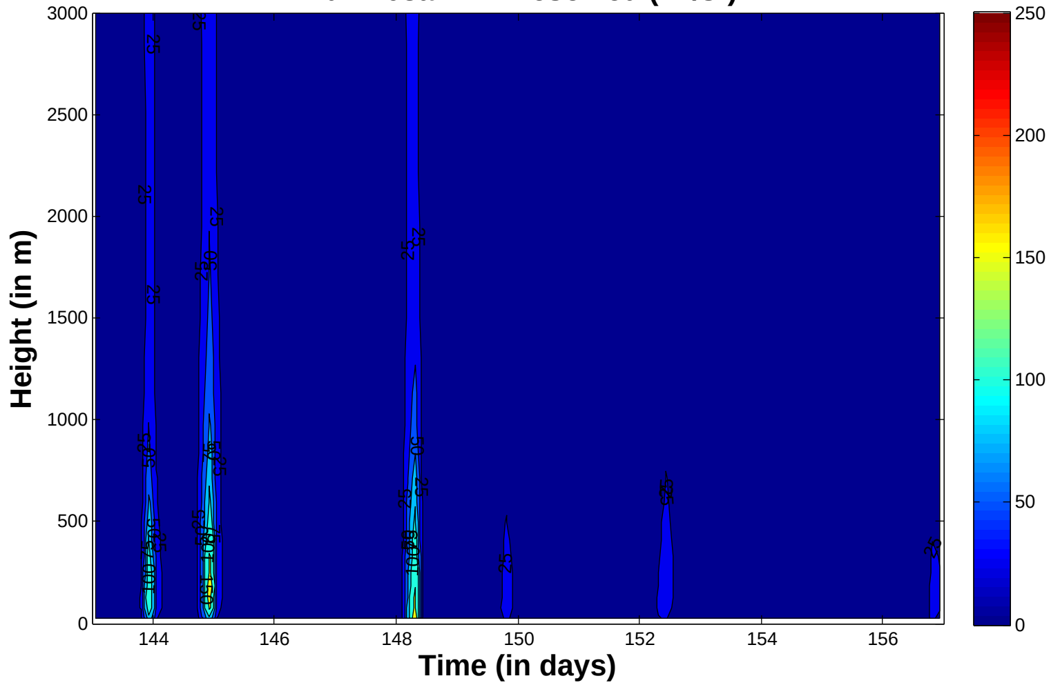
Run 208a TKE Resolved ( \text{m}^2/\text{s}^2 )
