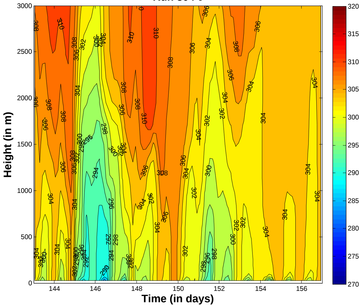
Run 304 \theta
