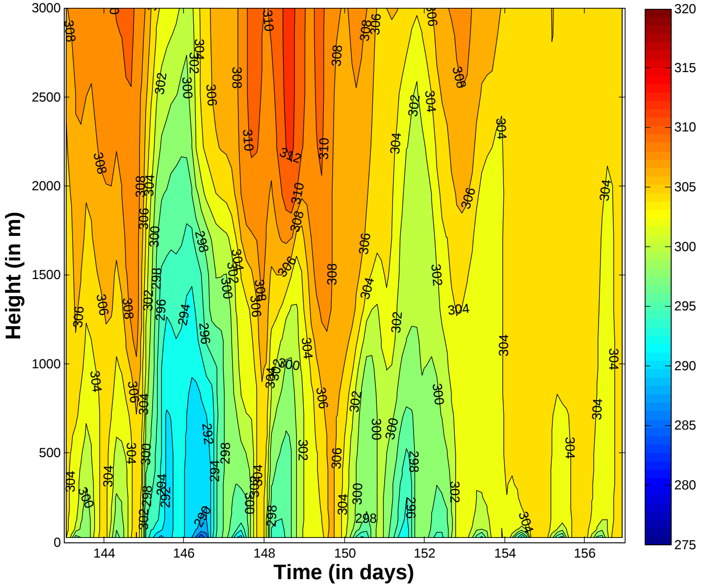
Run 306 \theta
