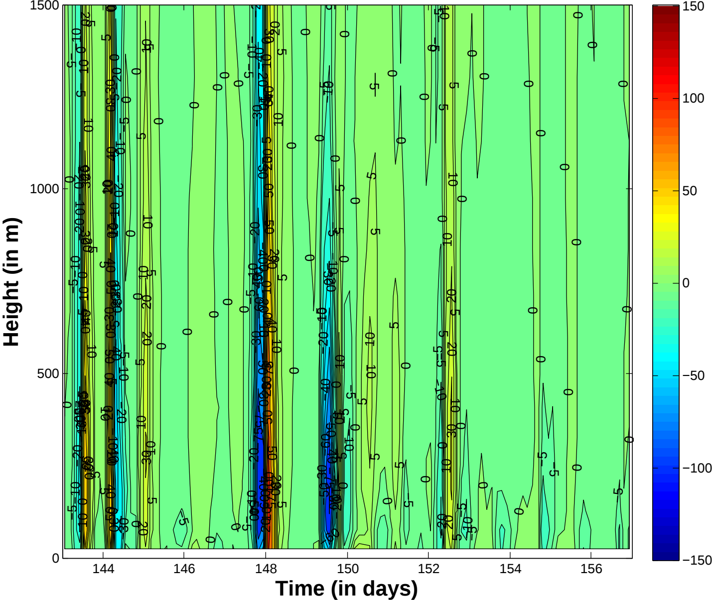
Run 306 – 206 Total TKE ( \text{m}^2/\text{s}^2 )
