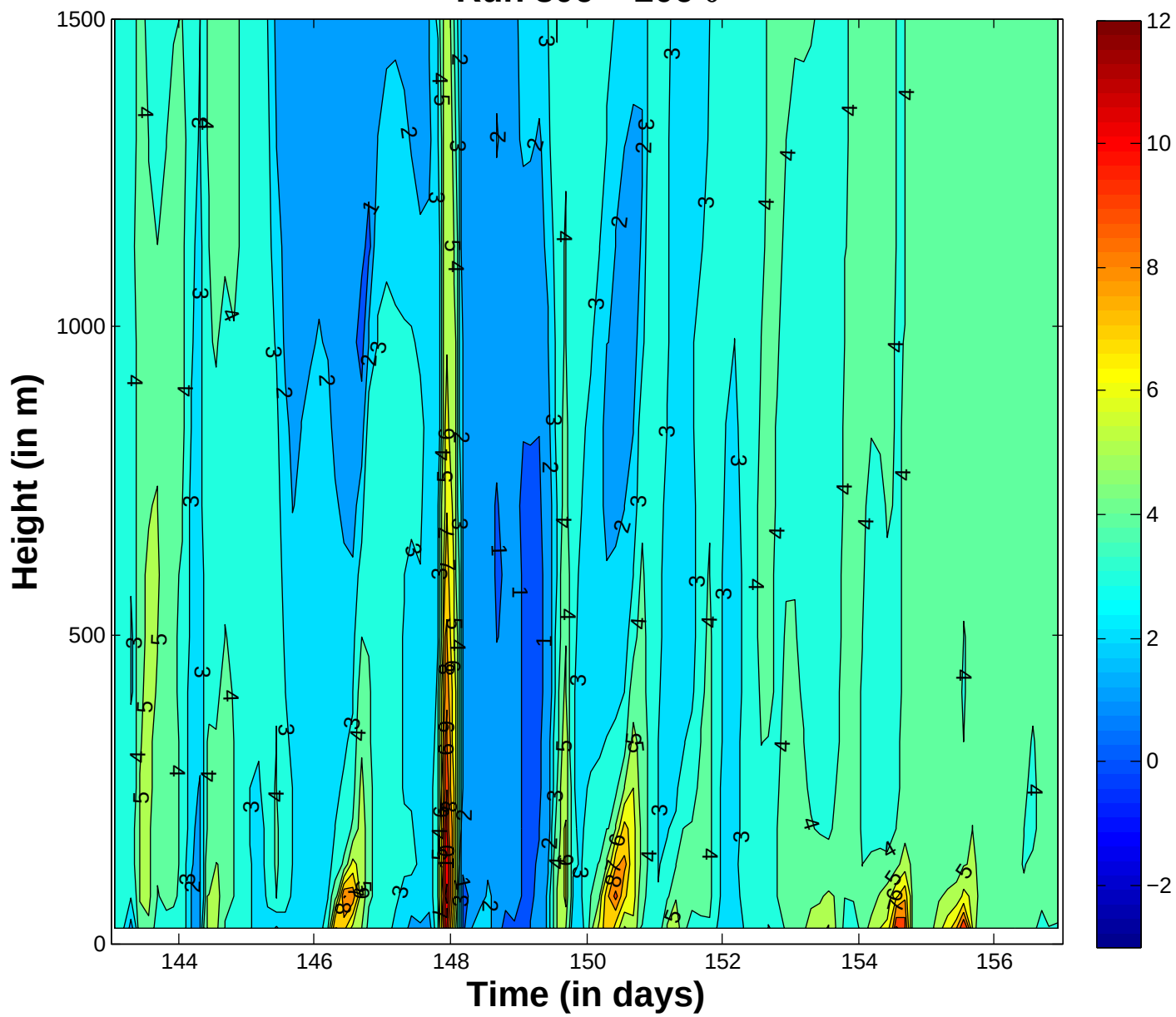
Run 306 – 206 \theta
