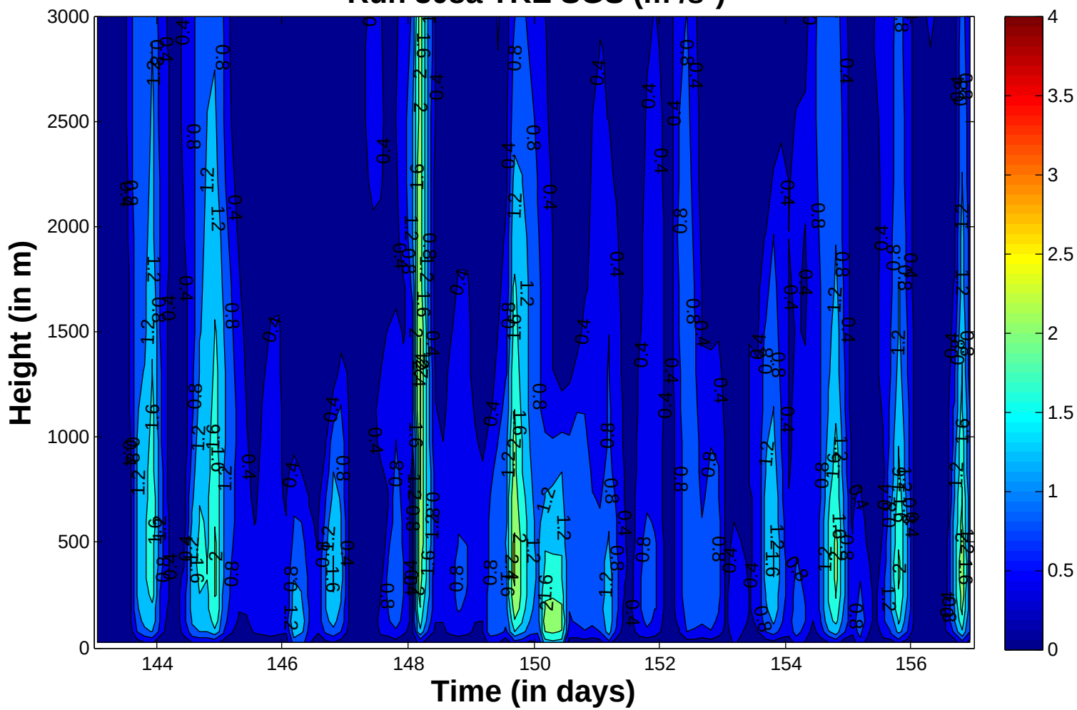
Run 308a TKE SGS ( \text{m}^2/\text{s}^2 )
