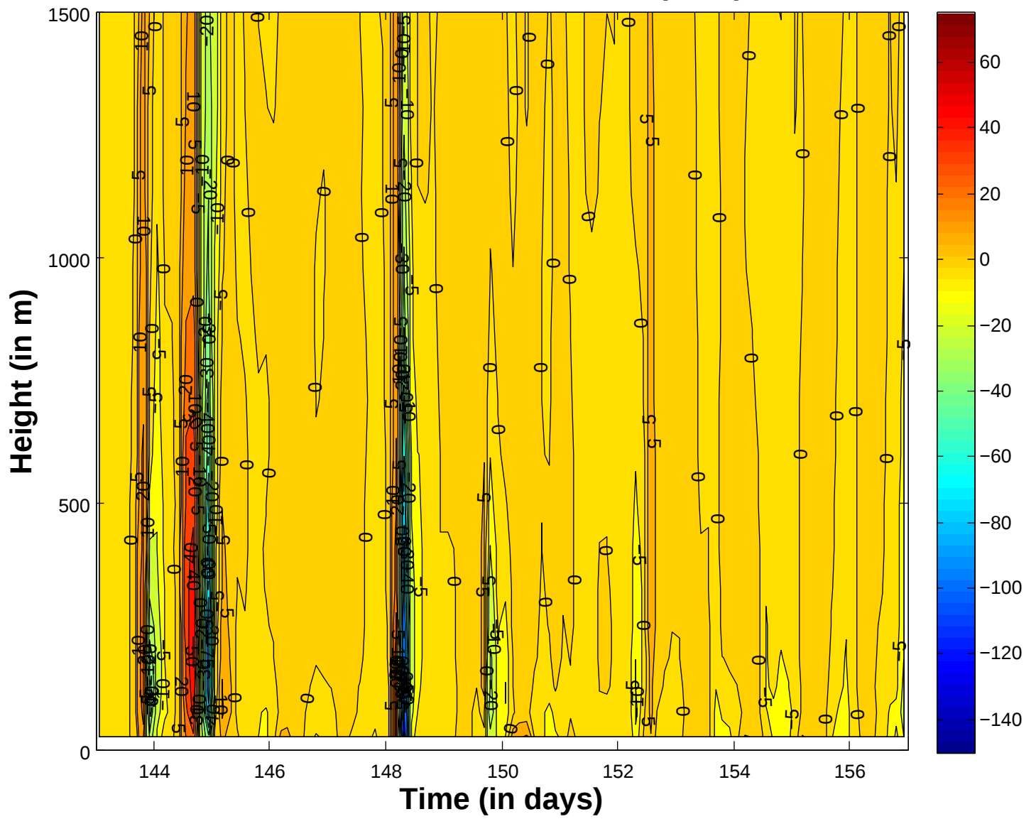
Run 308a – 208a Total TKE ( \text{m}^2/\text{s}^2 )
