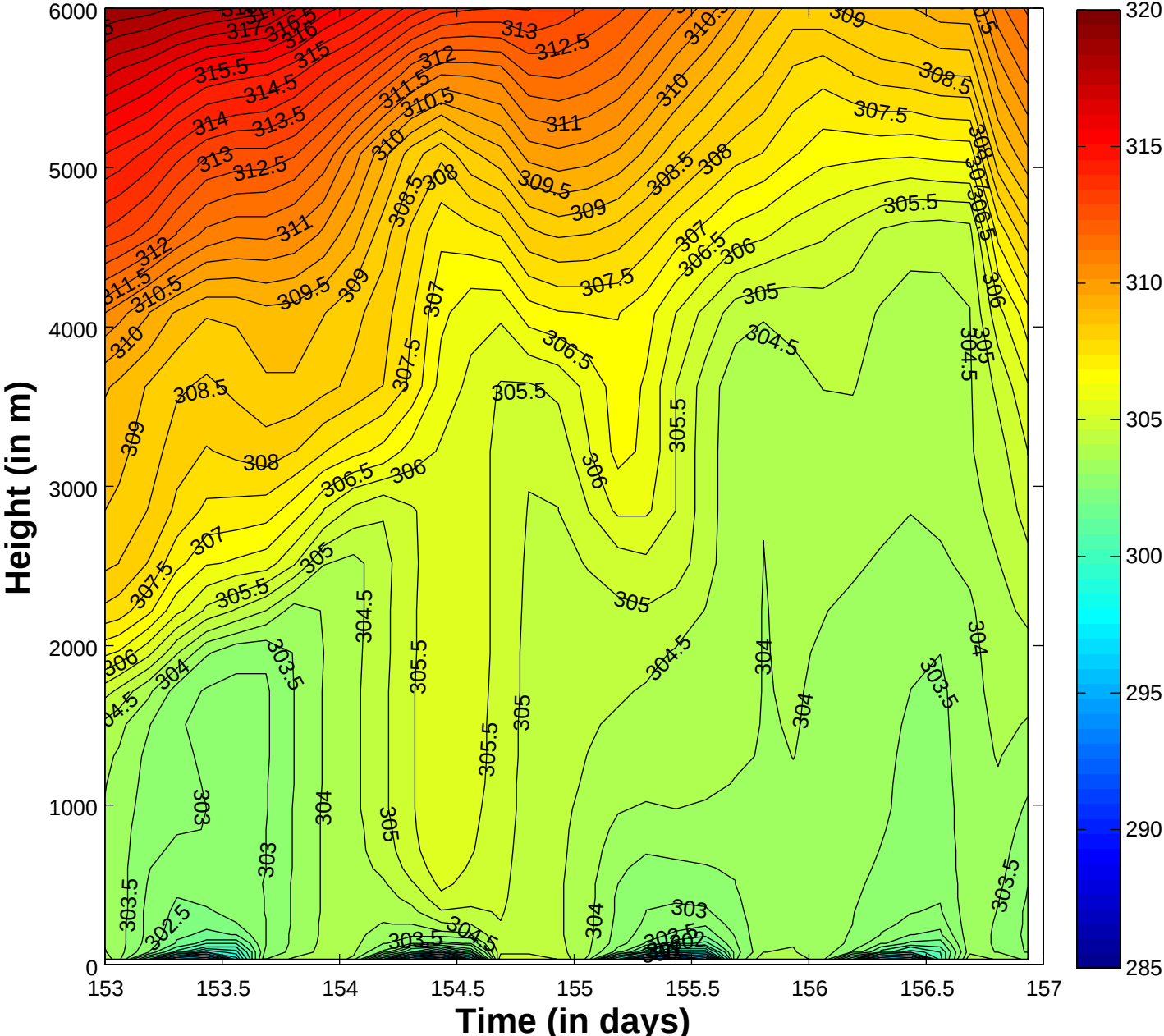
Run 208a \theta v
