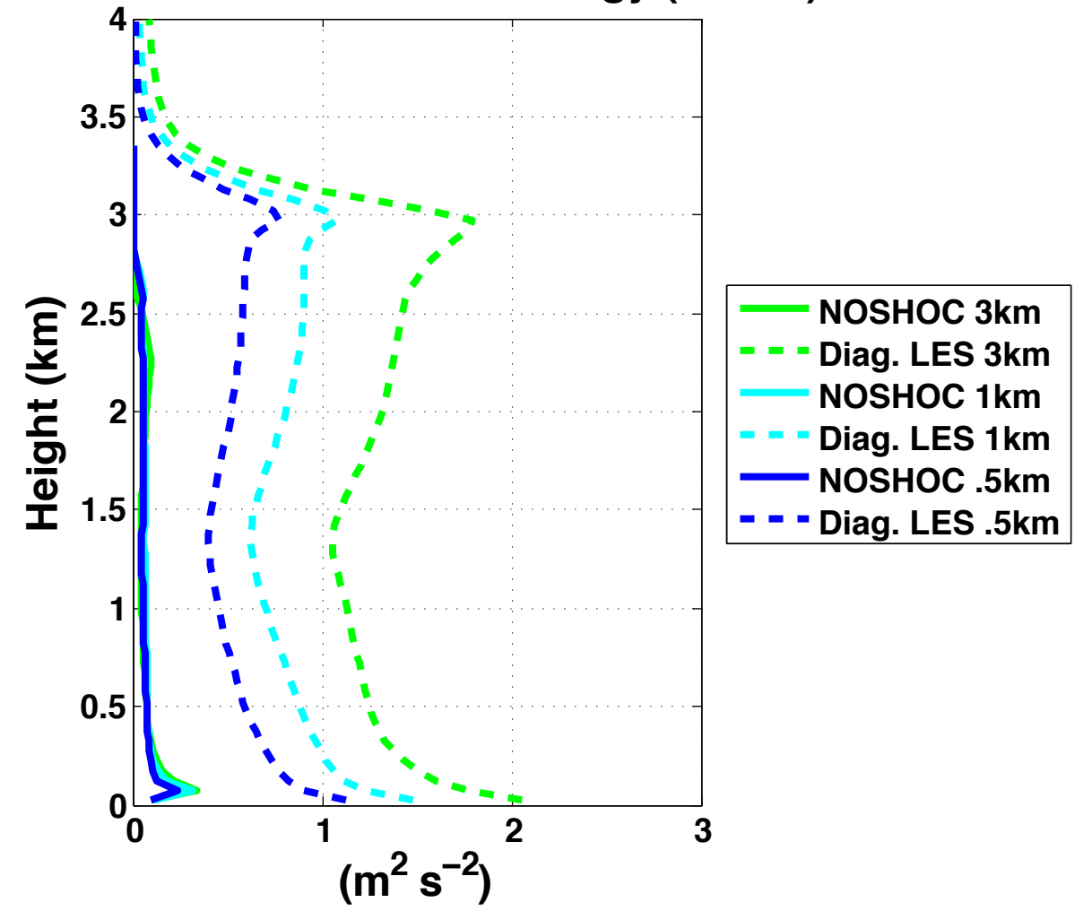
Total Turbulent Kinetic Energy (No Ice)
