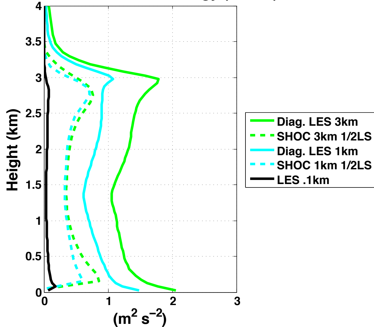
SGS Turbulent Kinetic Energy (No Ice)
