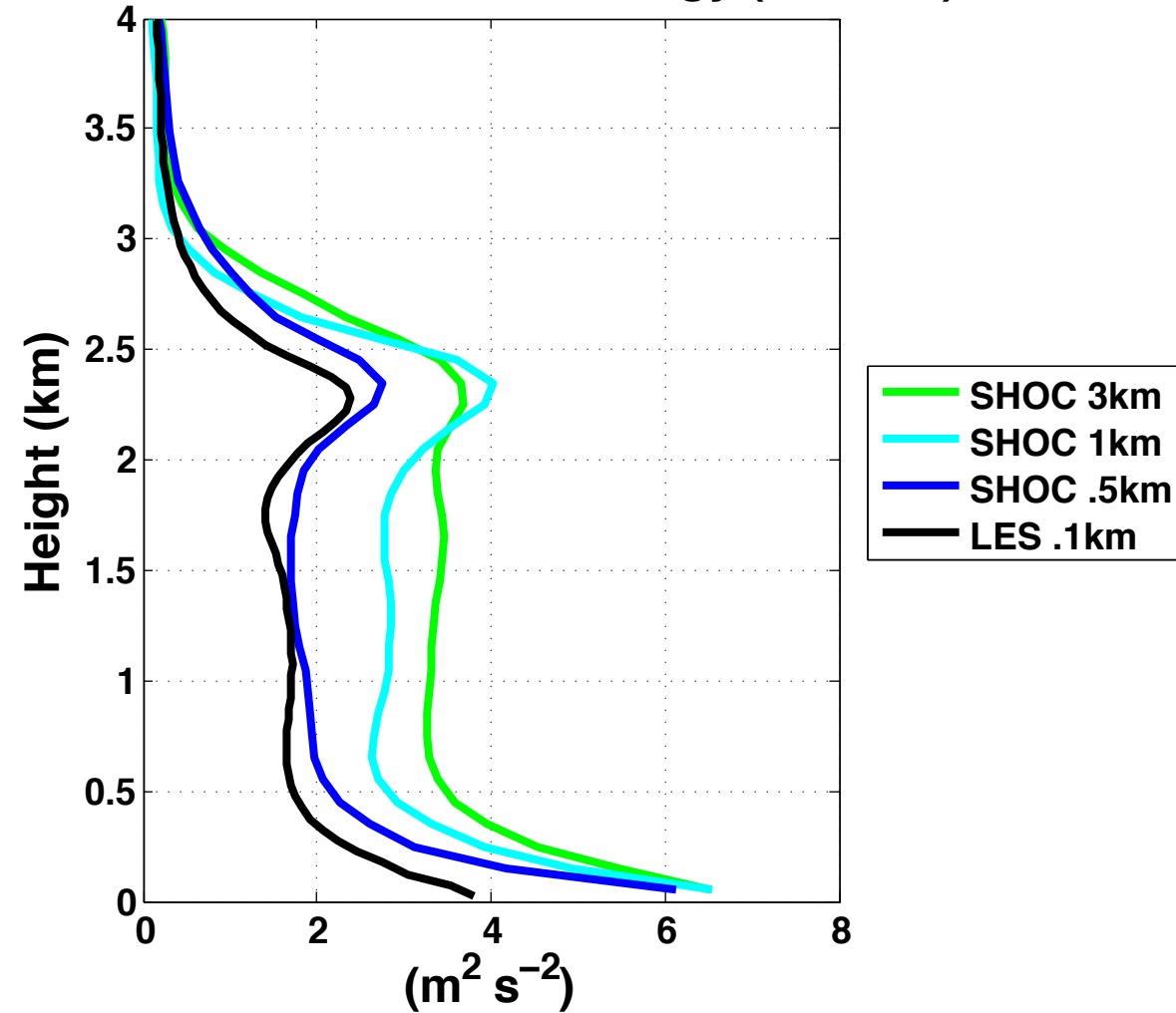
Total Turbulent Kinetic Energy (No Sed.)
