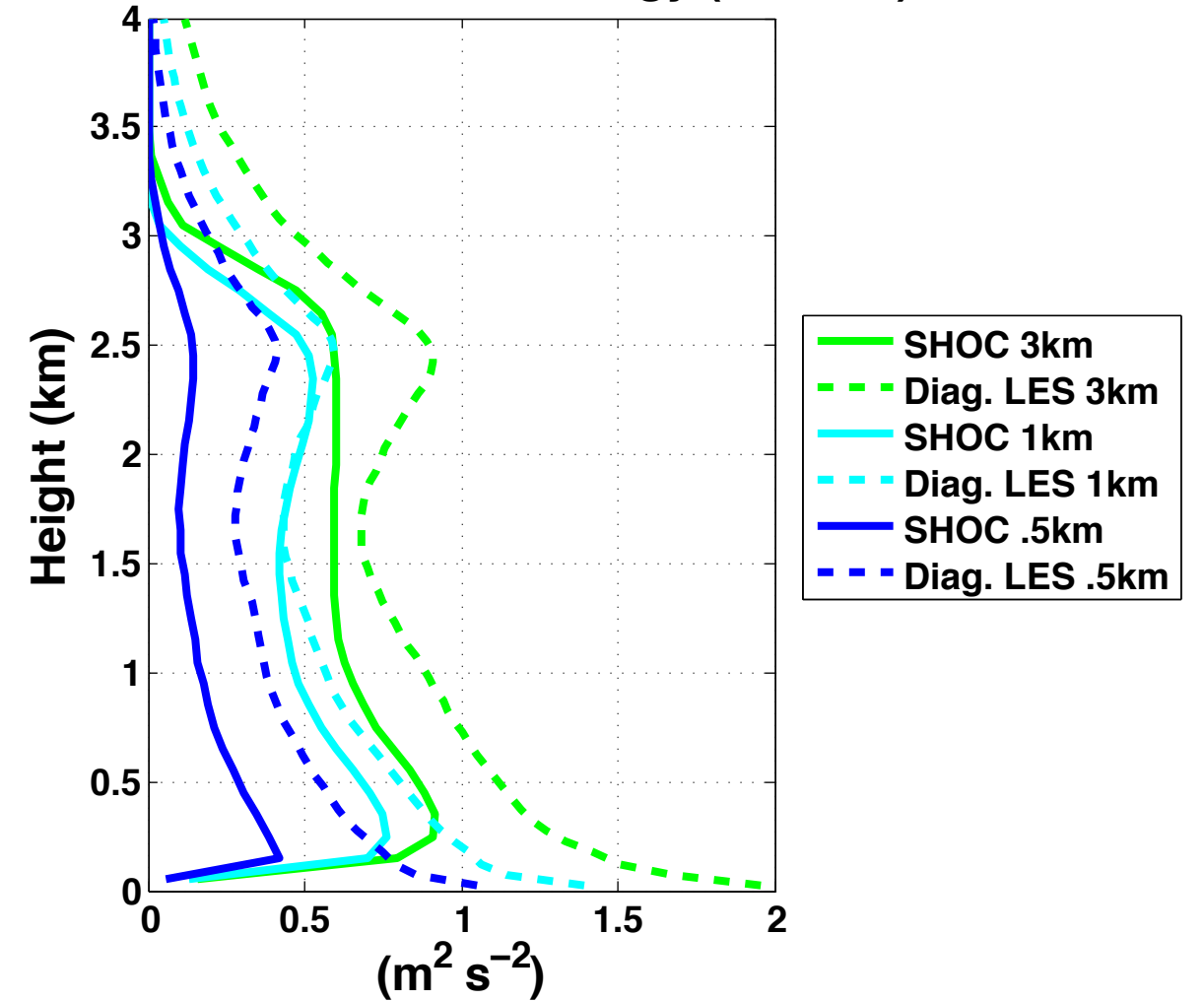
SGS Turbulent Kinetic Energy (No Sed.)
