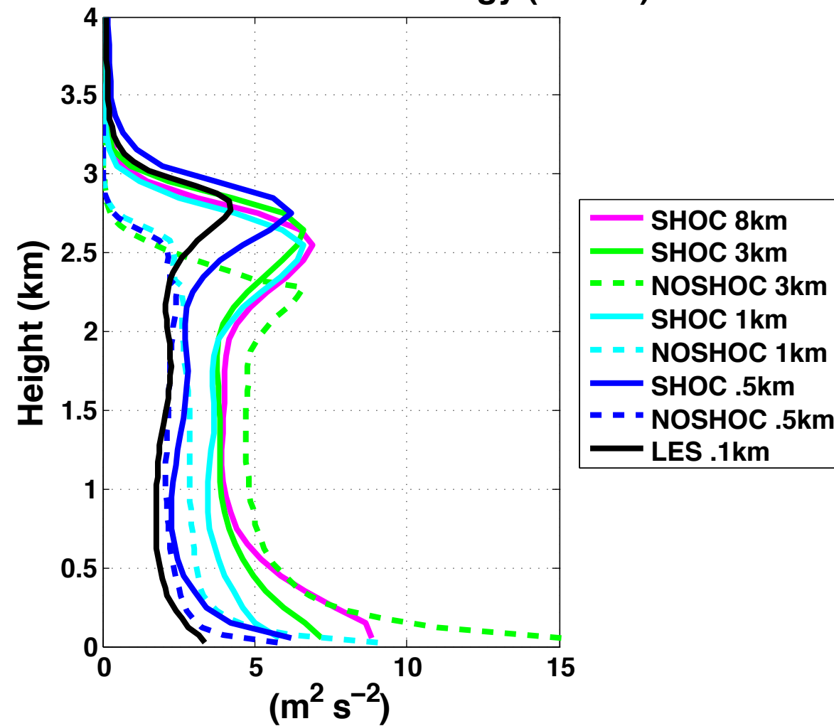
Total Turbulent Kinetic Energy (No Ice)
