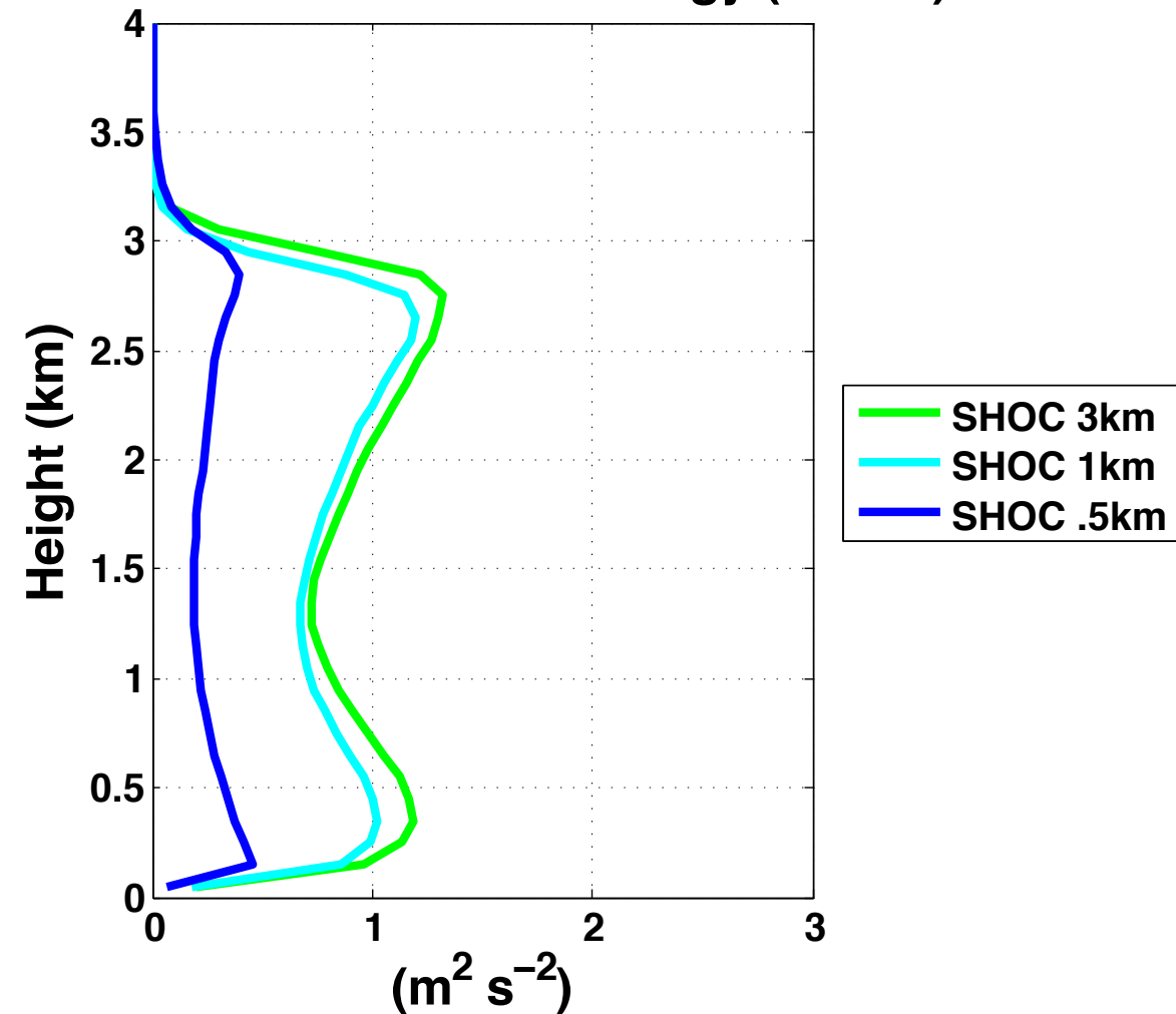
SGS Turbulent Kinetic Energy (No Ice)
