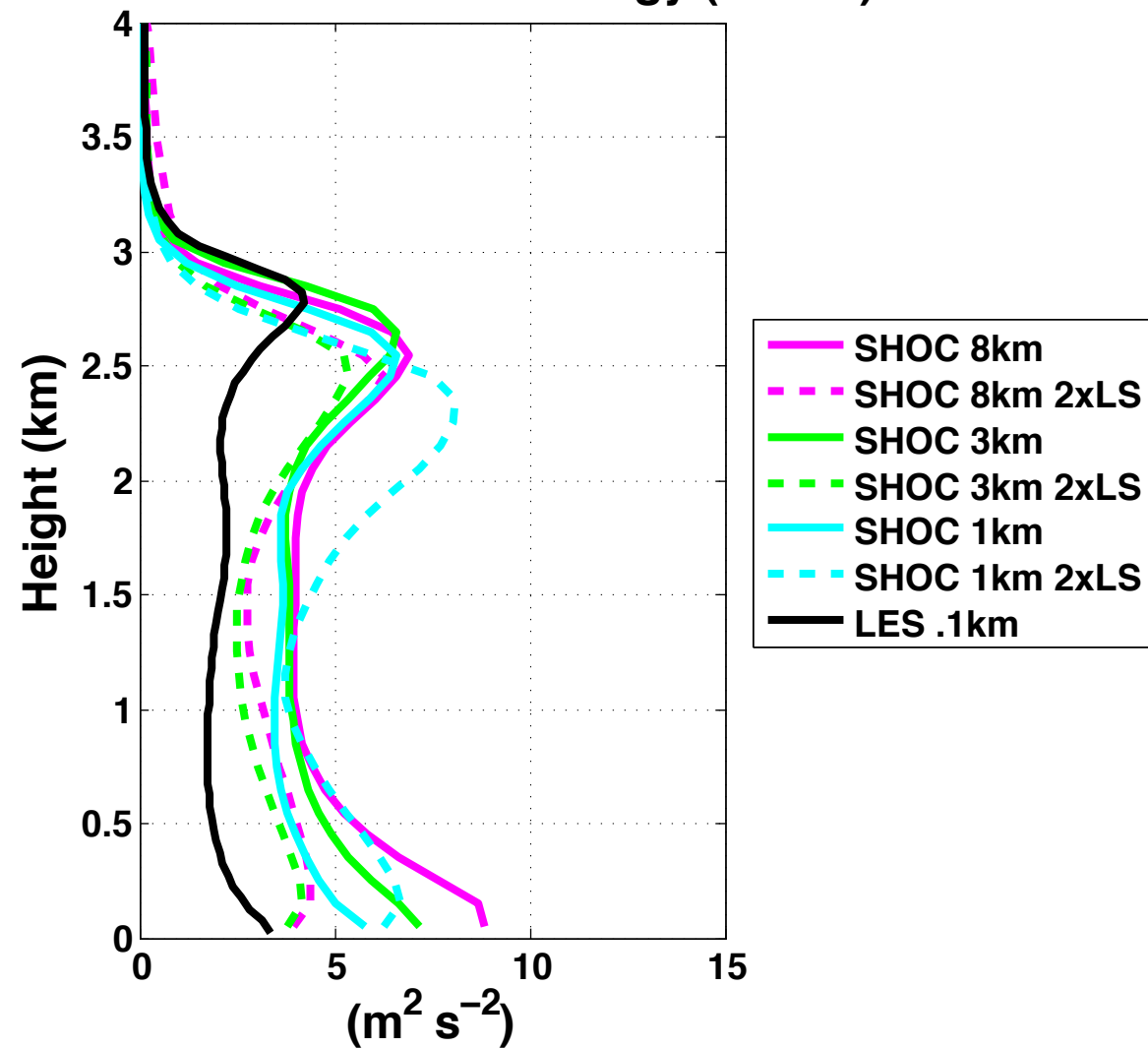
Total Turbulent Kinetic Energy (No Ice)
