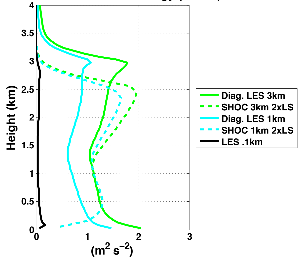
SGS Turbulent Kinetic Energy (No Ice)
