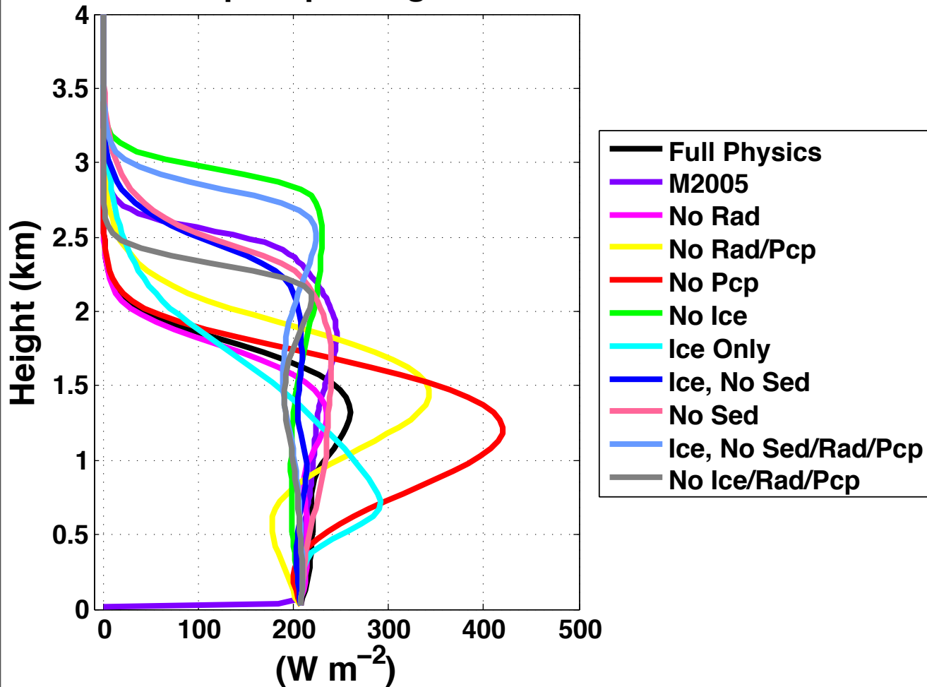
Total Nonprecipitating Water Flux
