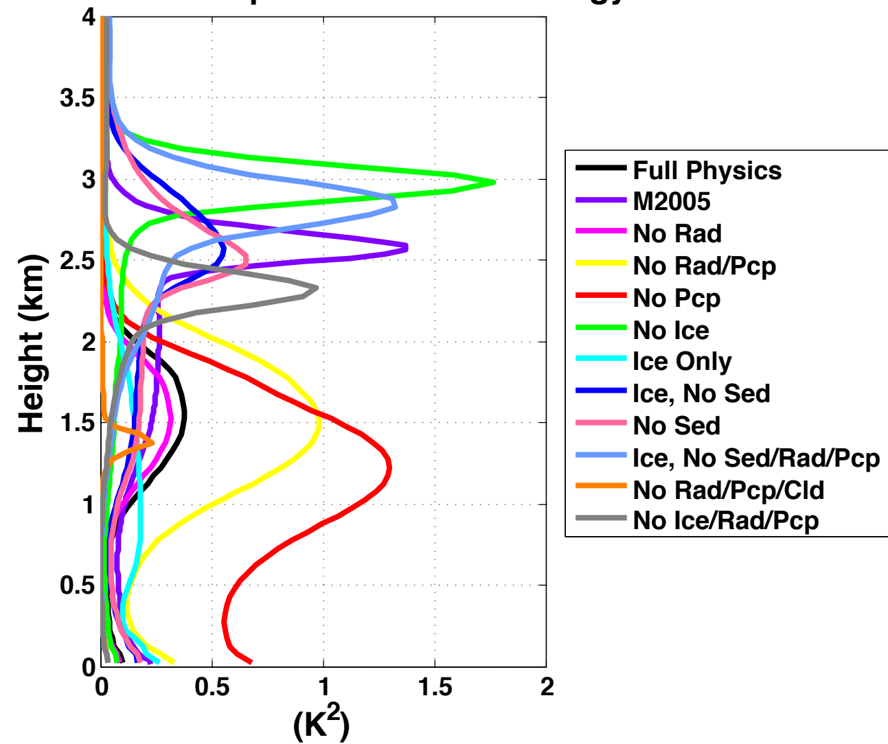
Variance of Liquid Water Static Energy
