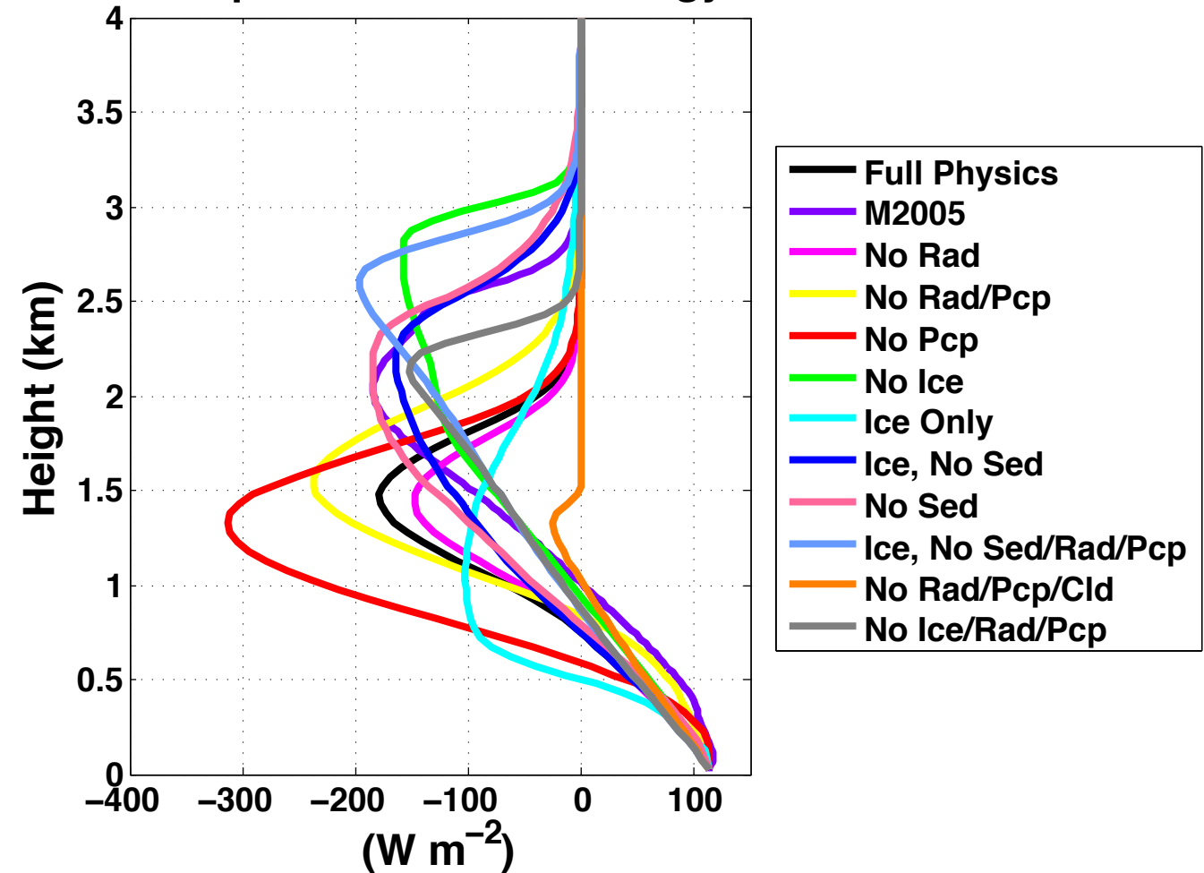
Total Liquid Water Static Energy Flux
