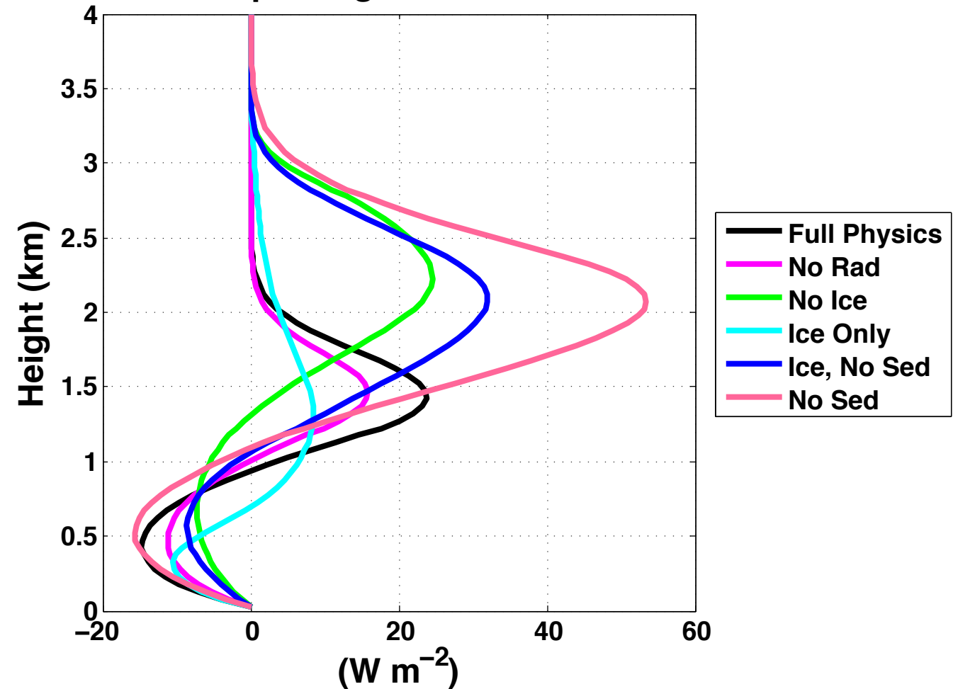
Total Precipitating-water Turbulent Flux
