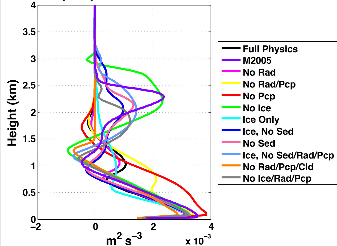
Total Buoyancy Production Terms of TKE
