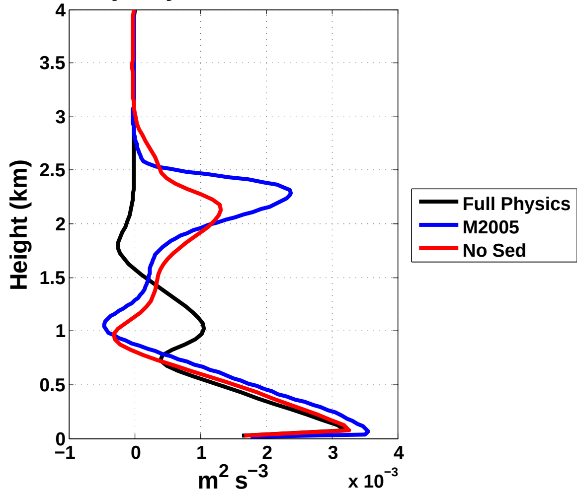
Total Buoyancy Production Terms of TKE
