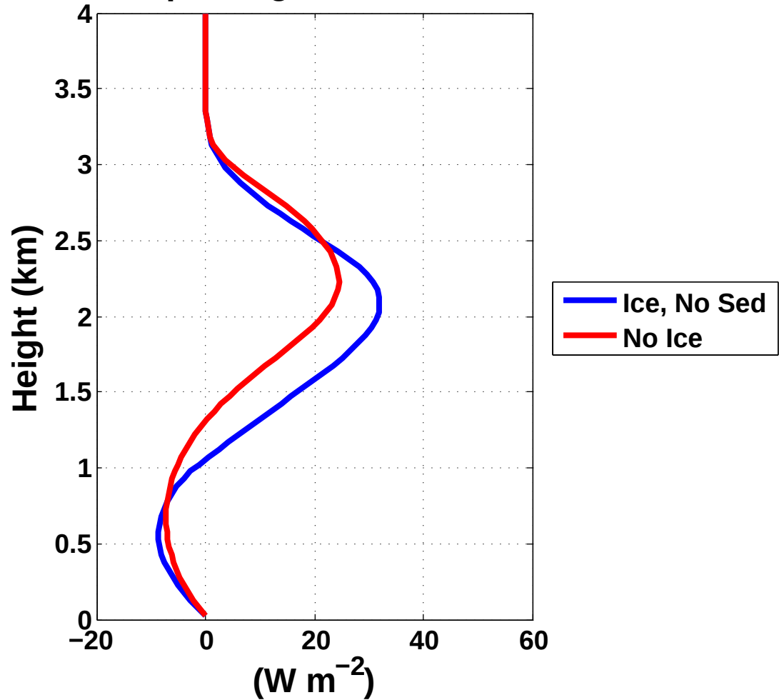
Total Precipitating-water Turbulent Flux
