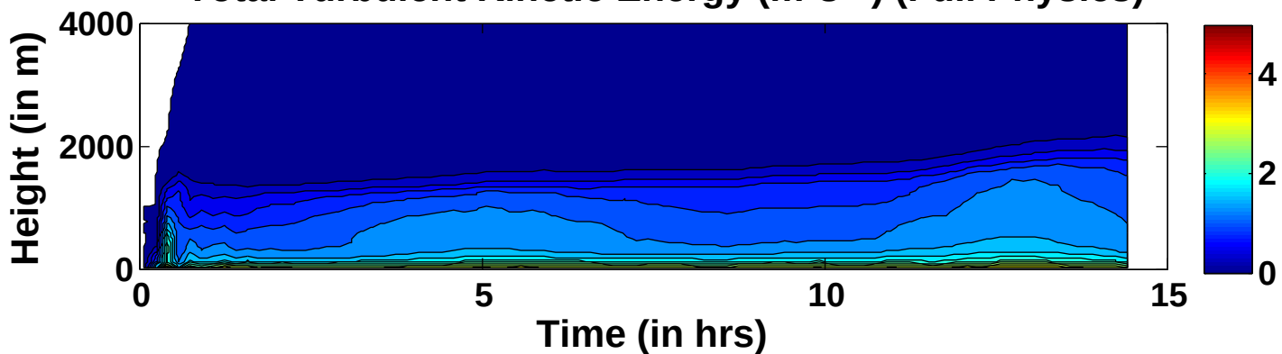
Total Turbulent Kinetic Energy ( \text{m}^2 \text{s}^{-2} ) (No Ice)
