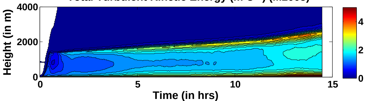
Total Turbulent Kinetic Energy ( \text{m}^2 \text{s}^{-2} ) (M2005)
