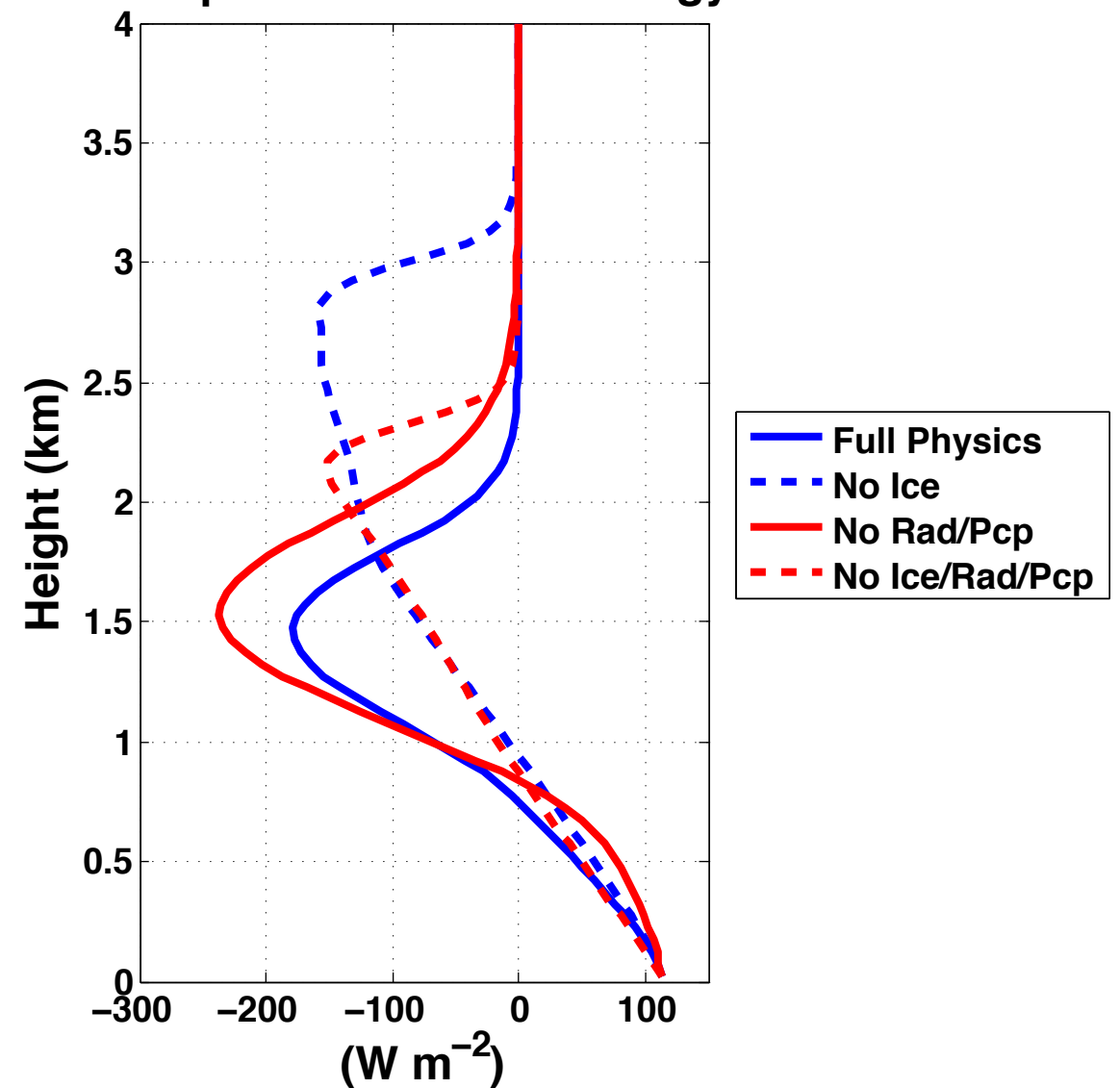
Total Liquid Water Static Energy Flux
