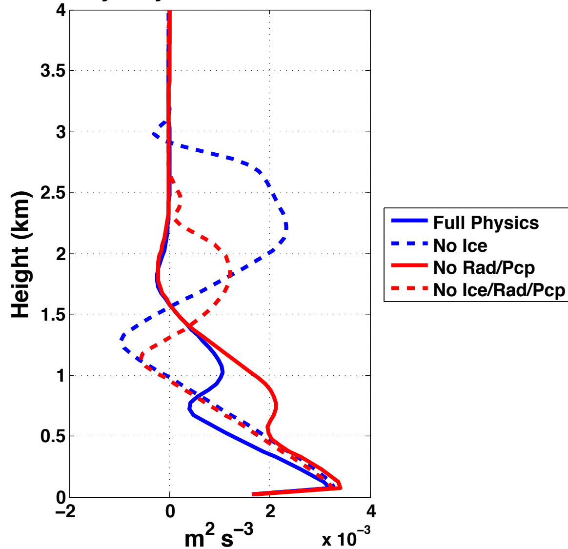
Total Buoyancy Production Terms of TKE
