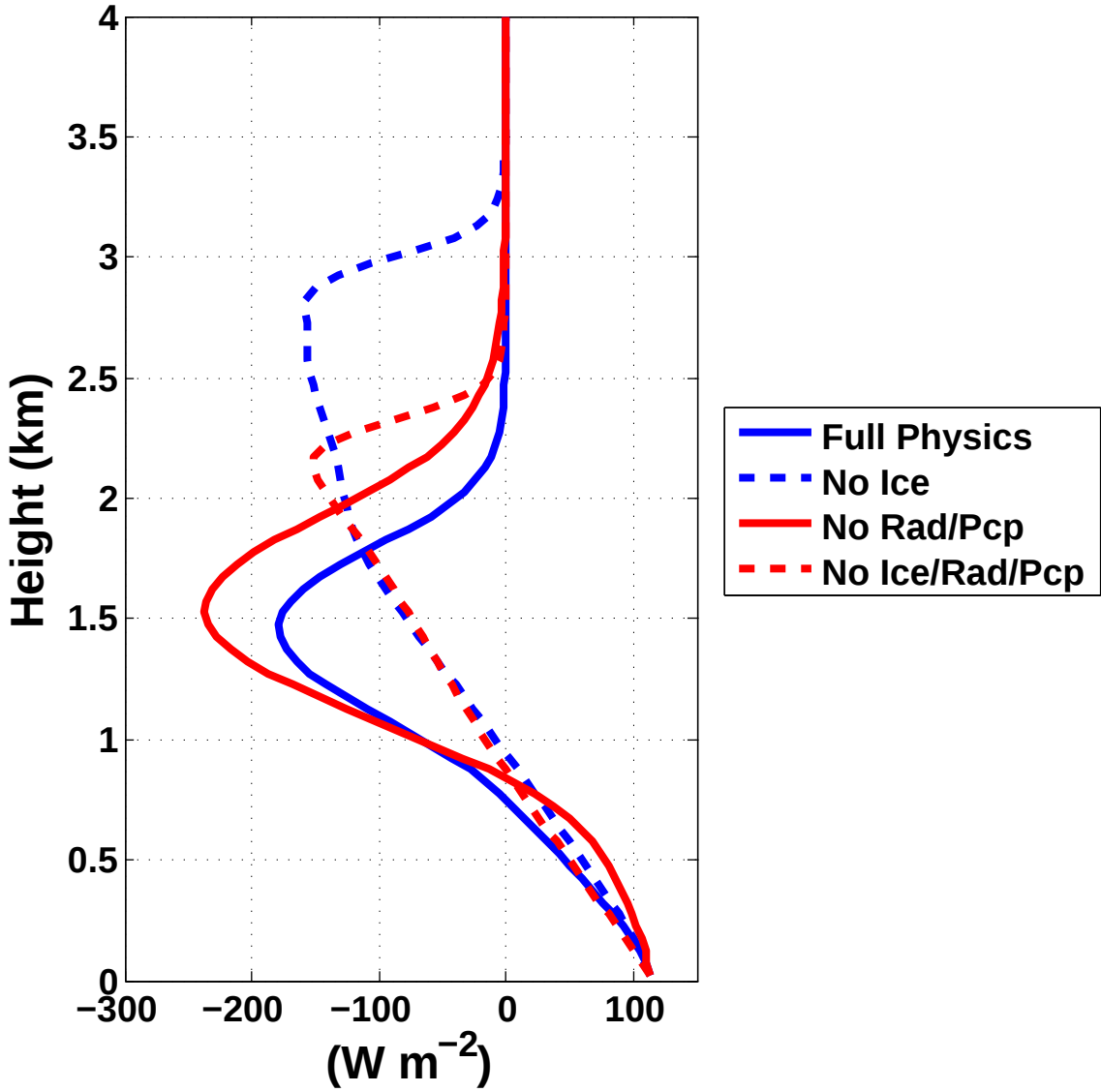
Total Liquid Water Static Energy Flux
