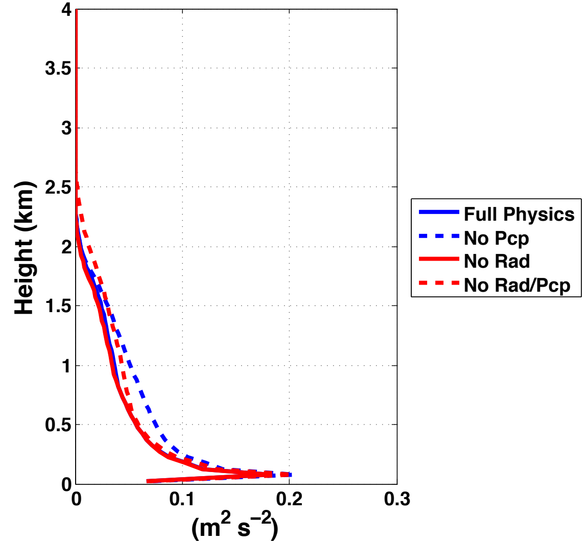
SGS Turbulent Kinetic Energy
