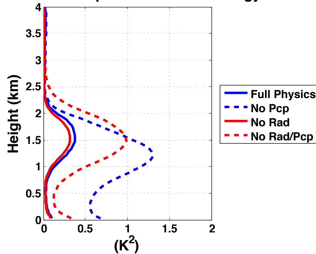
Variance of Liquid Water Static Energy
