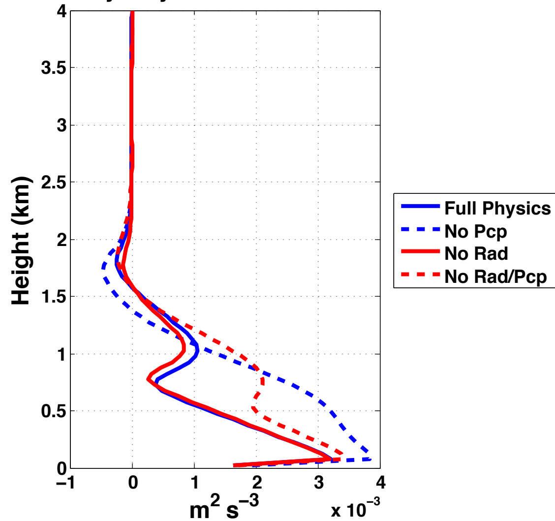
Total Buoyancy Production Terms of TKE
