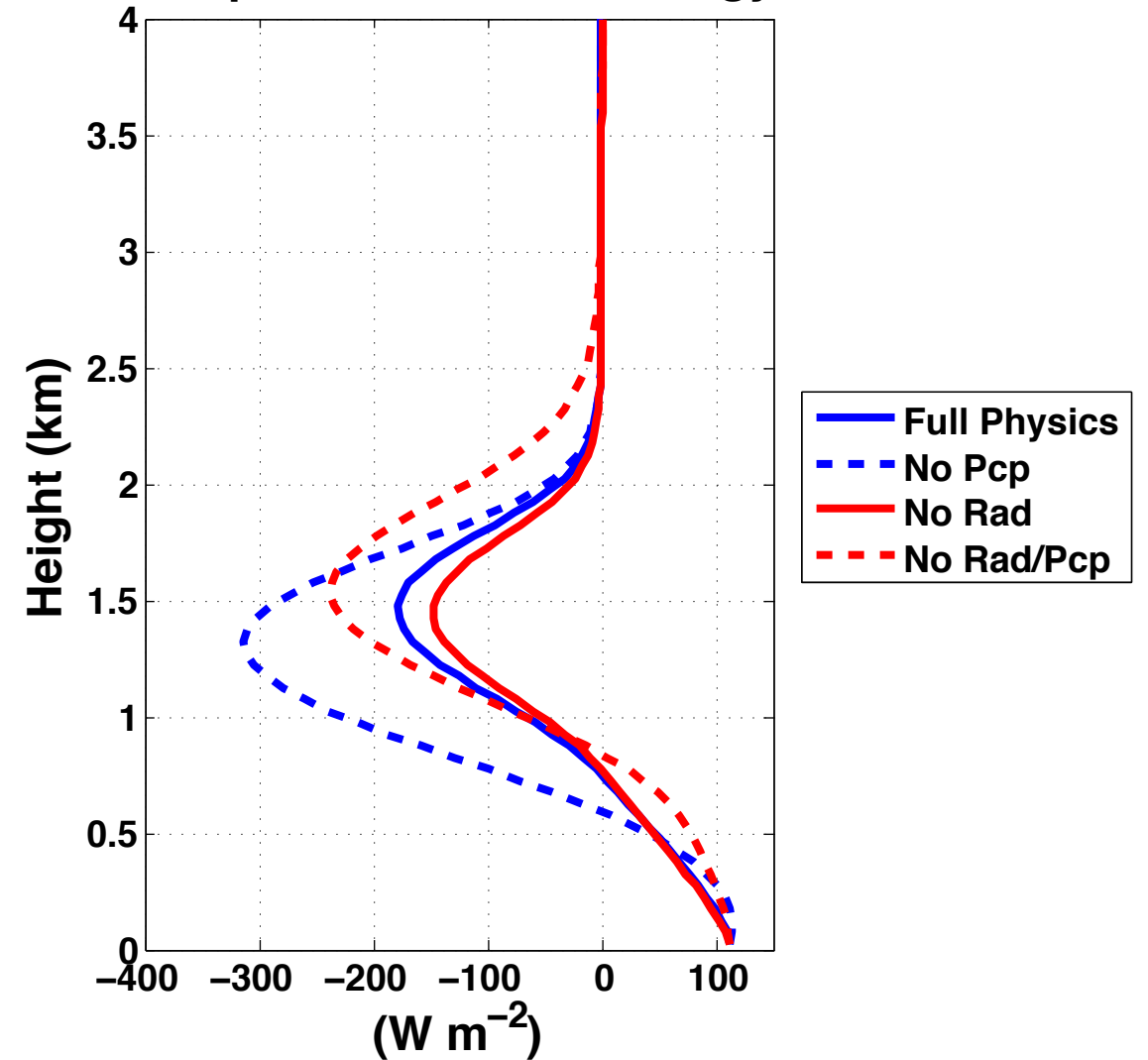
Total Liquid Water Static Energy Flux
