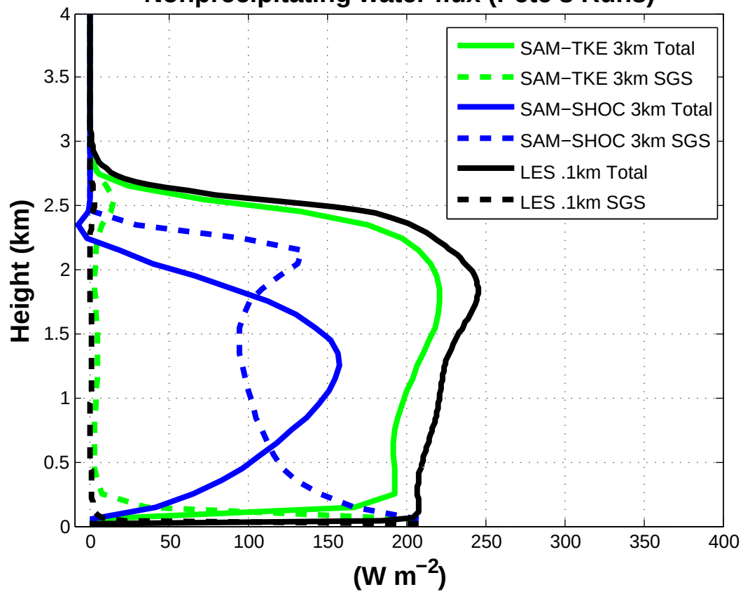
Nonprecipitating water flux (Pete's Runs)
