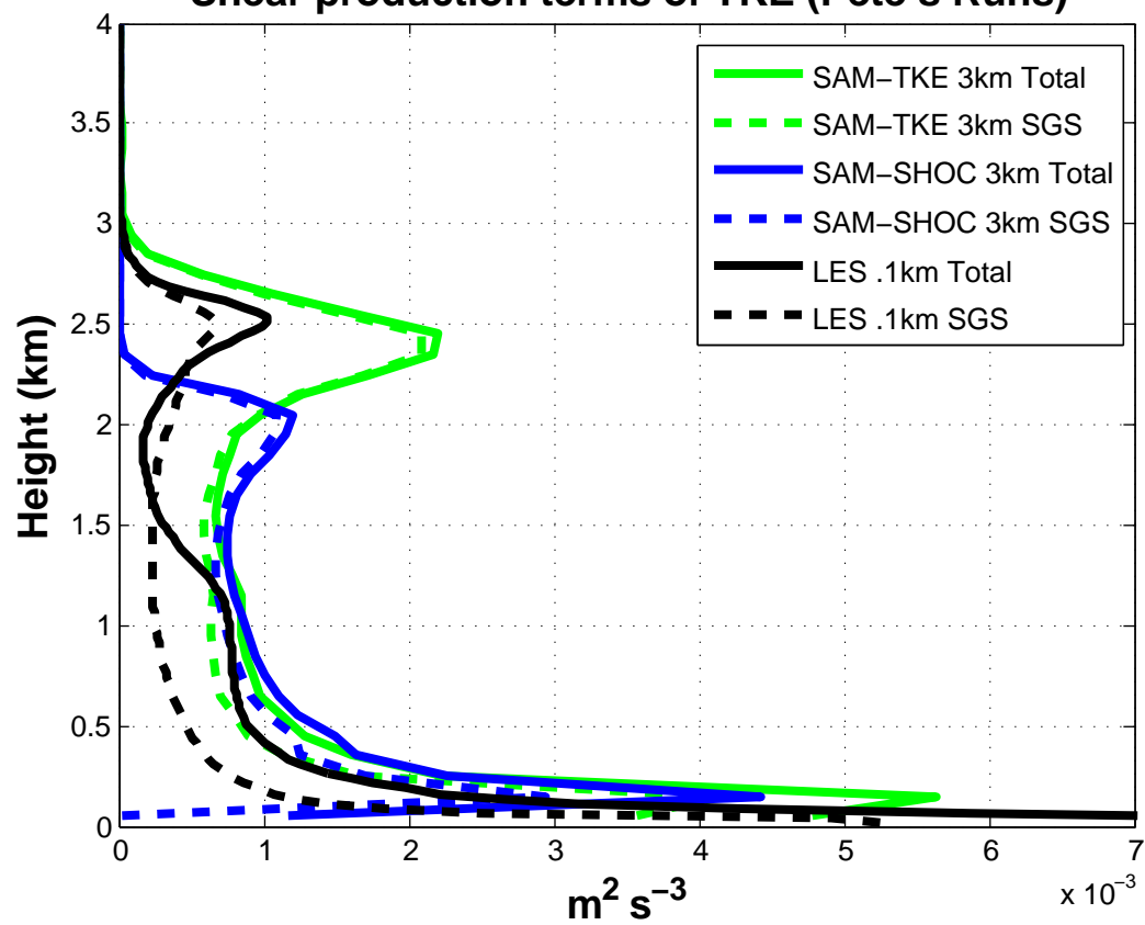
Shear production terms of TKE (Pete's Runs)
