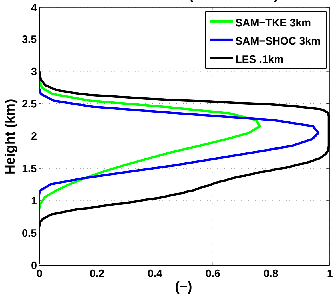
Cloud Fraction (M2005 Runs)
