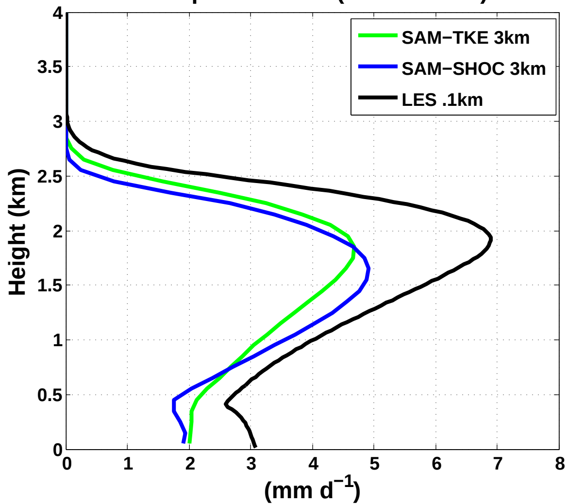
Precipitation Flux (M2005 Runs)
