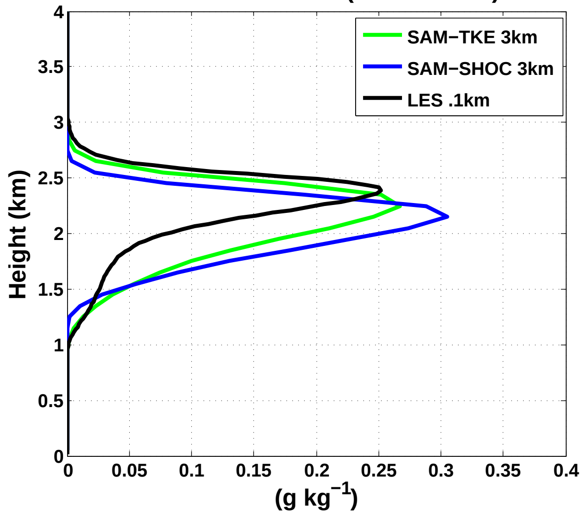
Total Cloud Water (M2005 Runs)
