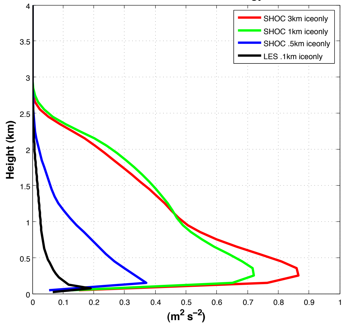
SGS Turbulent Kinetic Energy
