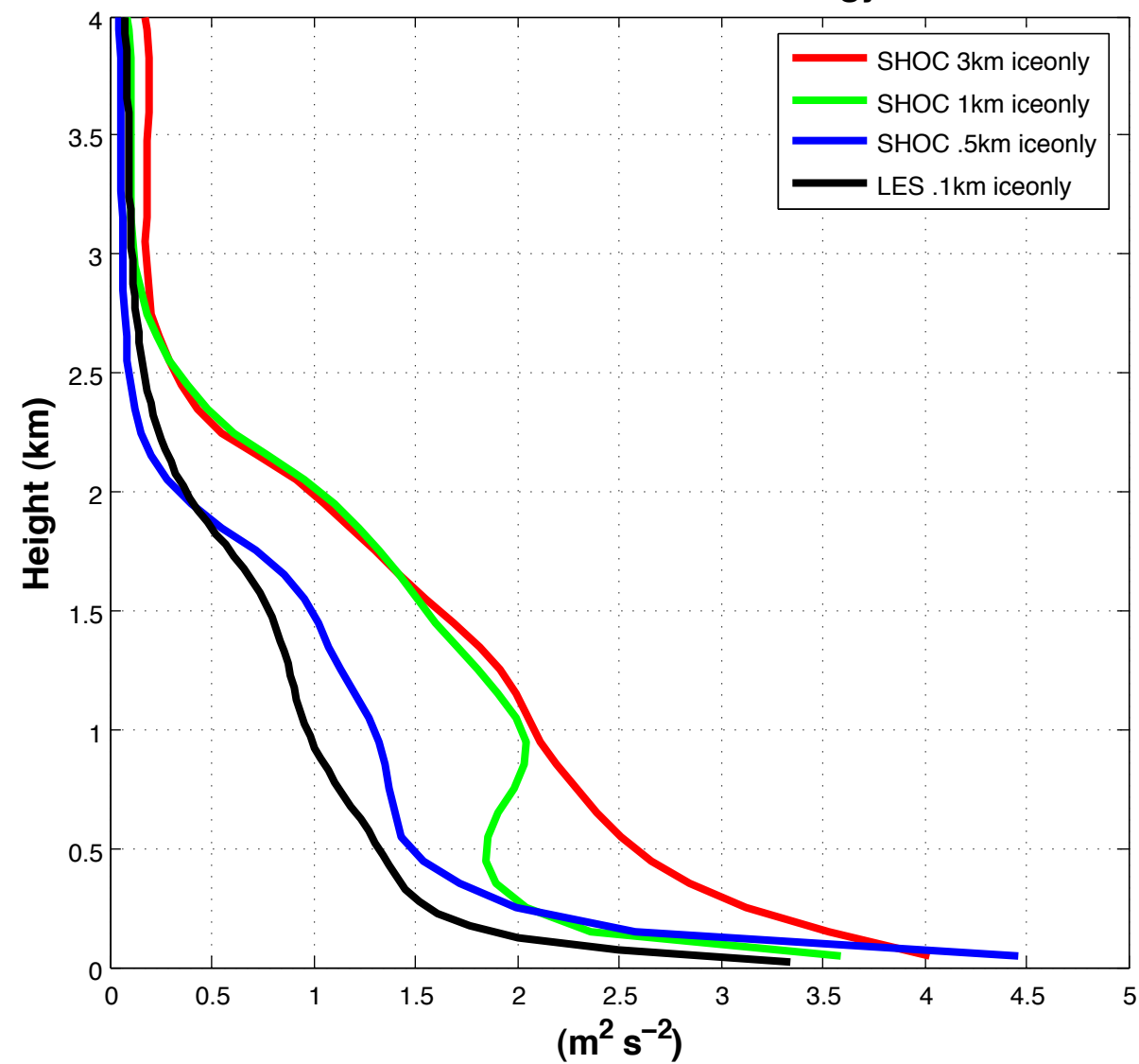
Total Turbulent Kinetic Energy
