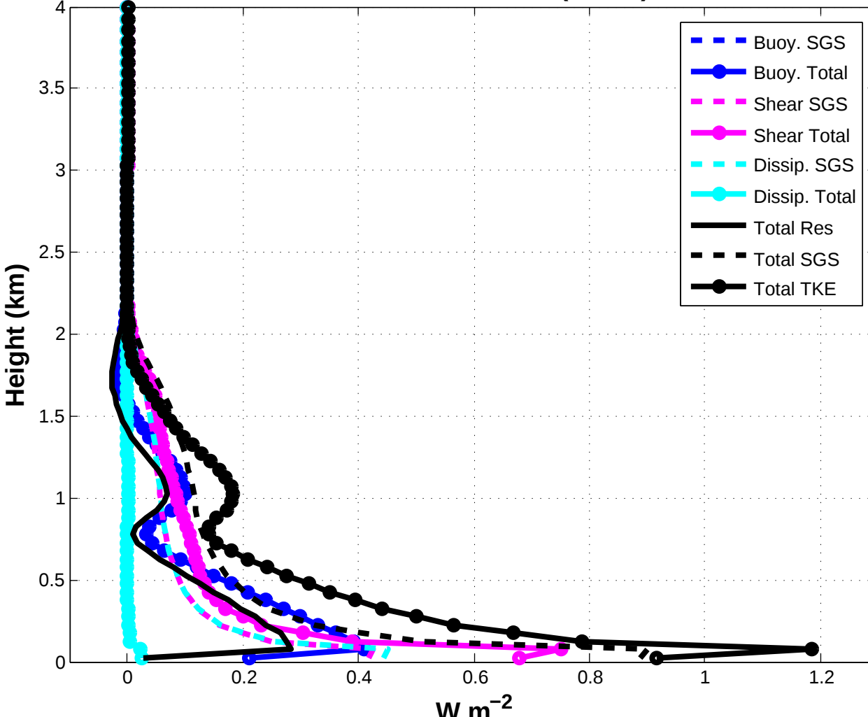
TKE terms .5km LES (norad)
