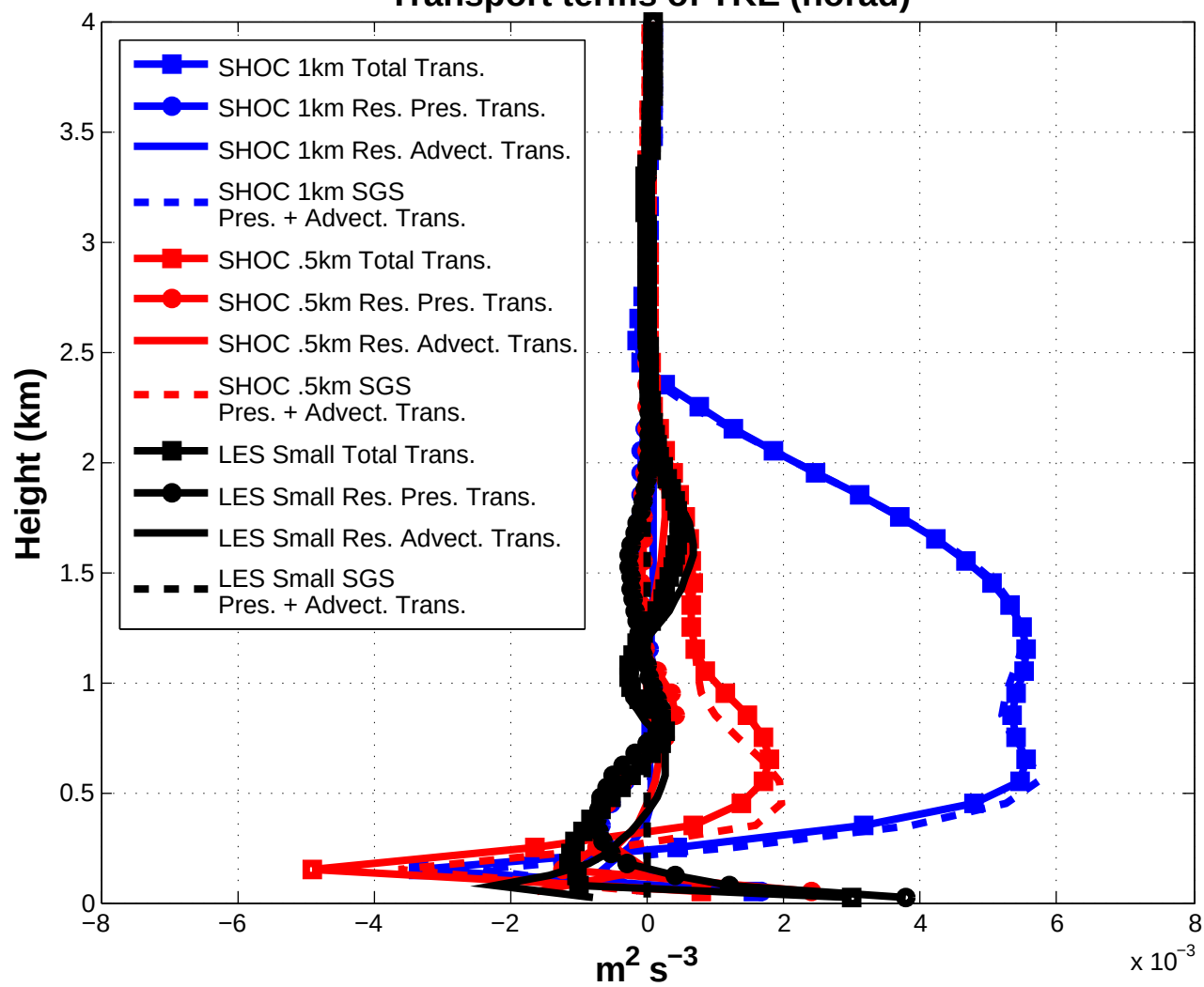
Transport terms of TKE (norad)
