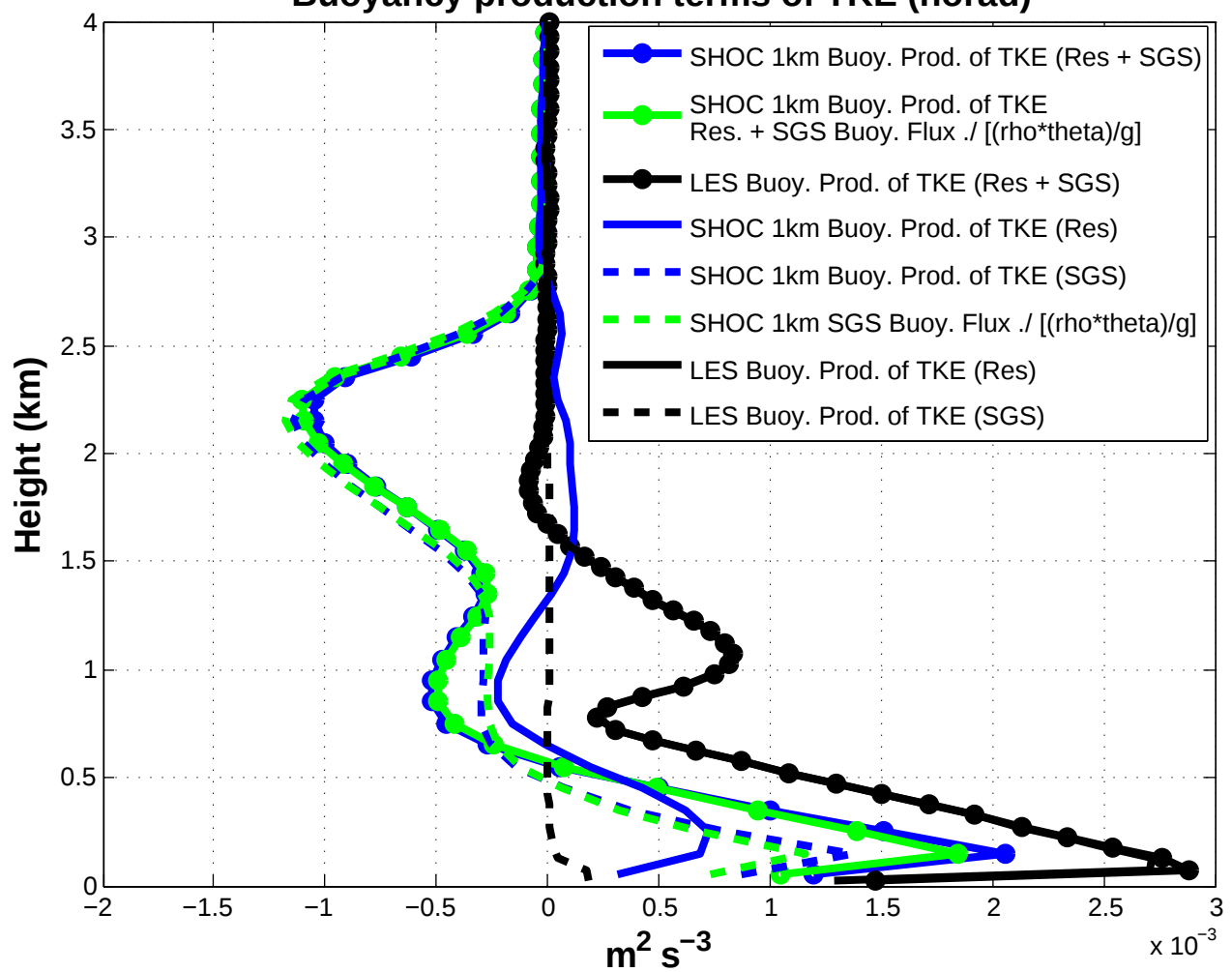
Buoyancy production terms of TKE (norad)
