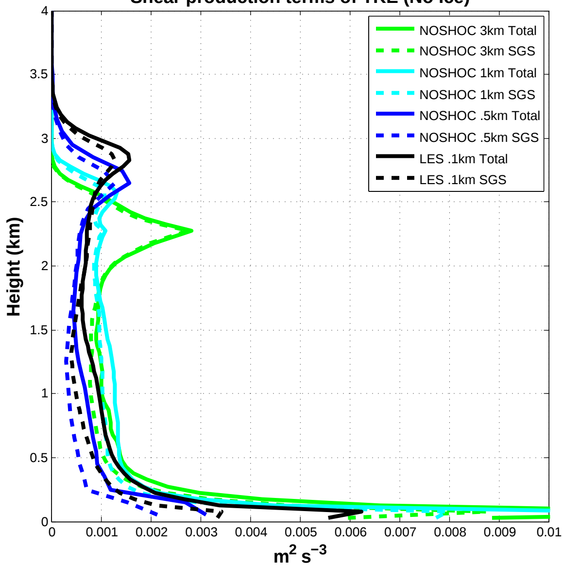
Shear production terms of TKE (No Ice)
