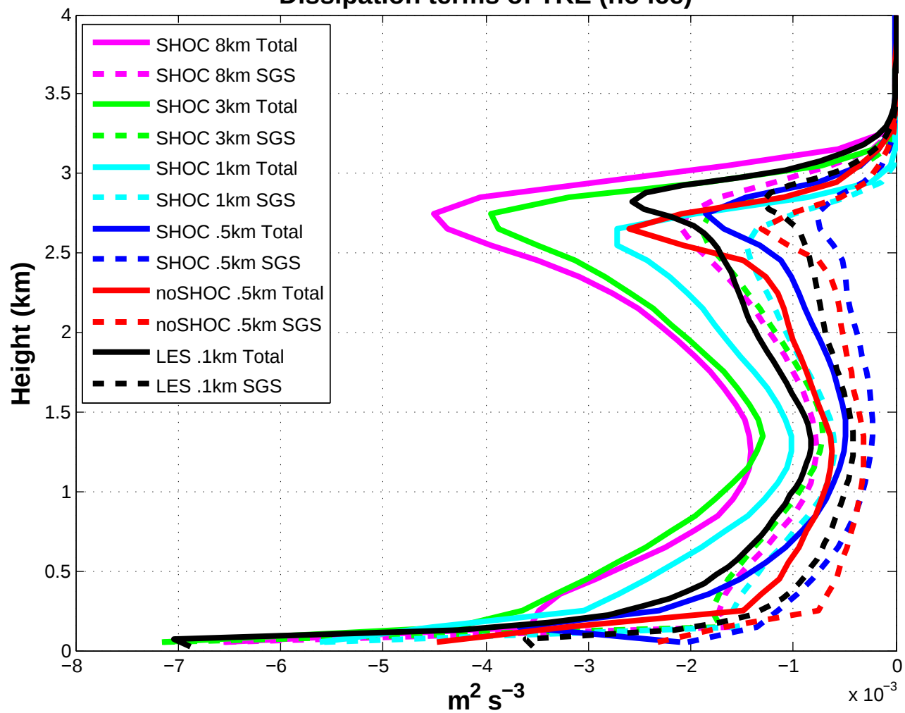
Dissipation terms of TKE (no ice)
