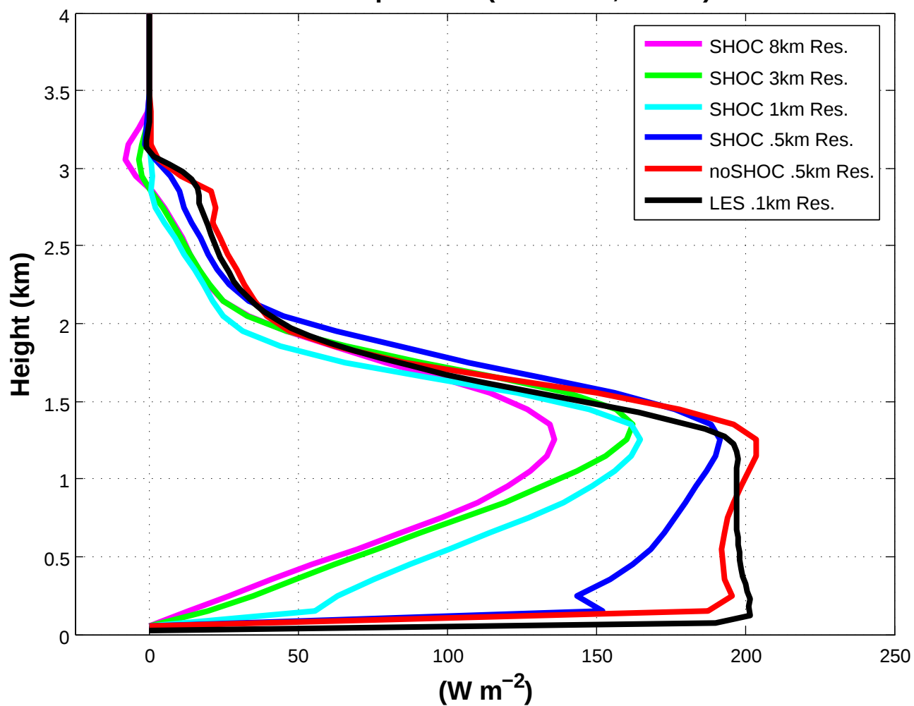
Water Vapor Flux (Resolved, no ice)
