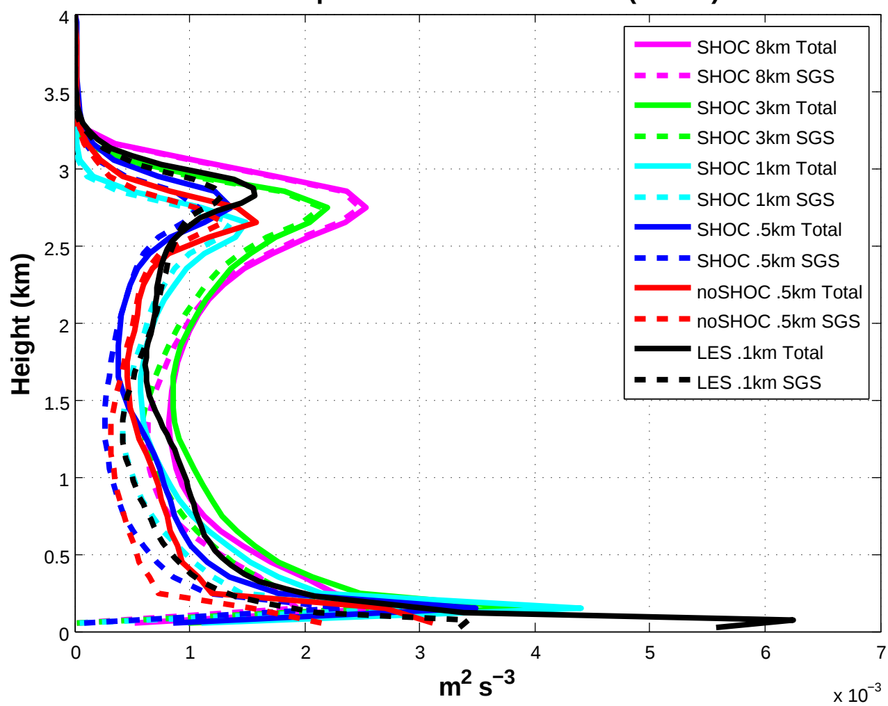
Shear production terms of TKE (no ice)
