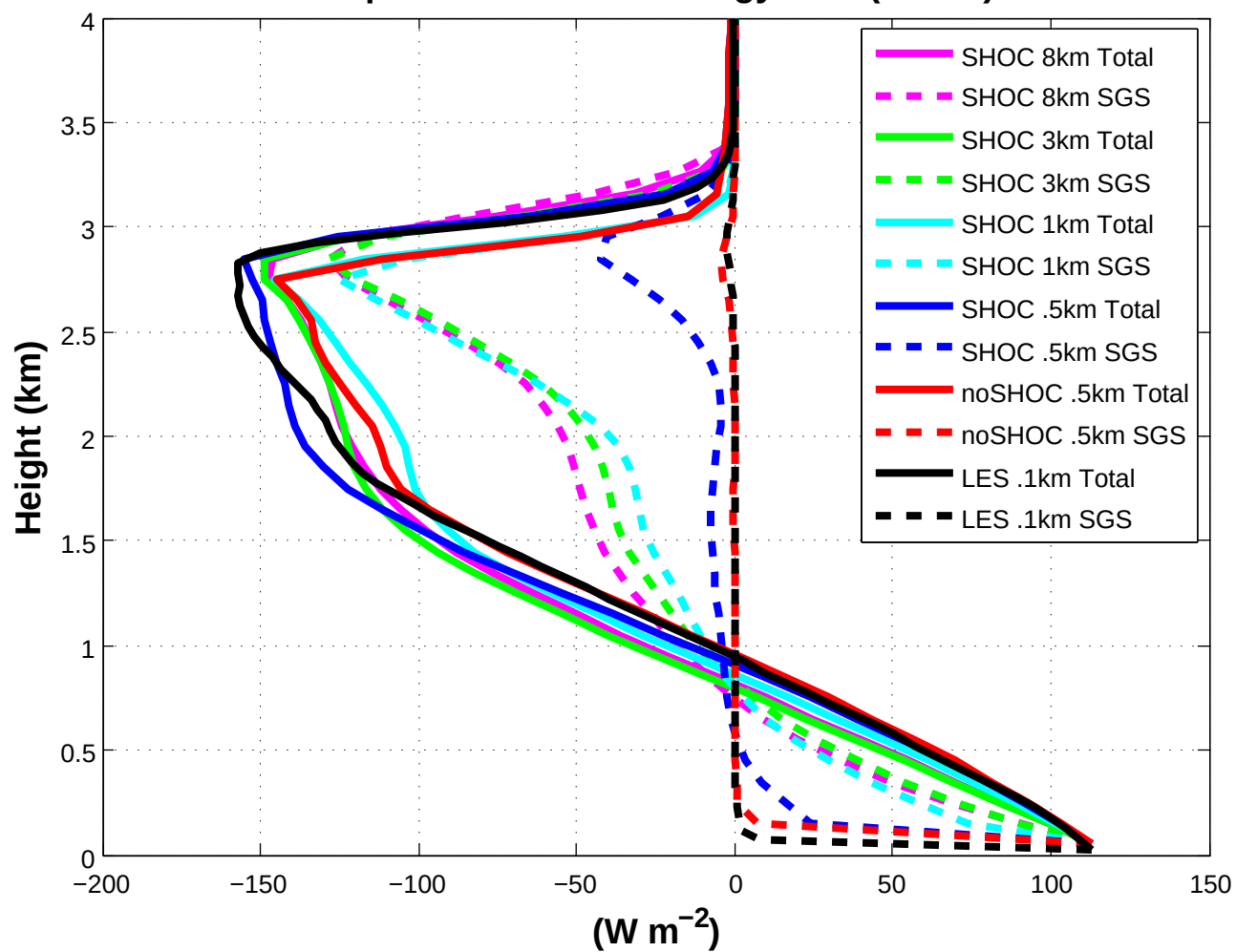
Liquid Water Static Energy Flux (no ice)
