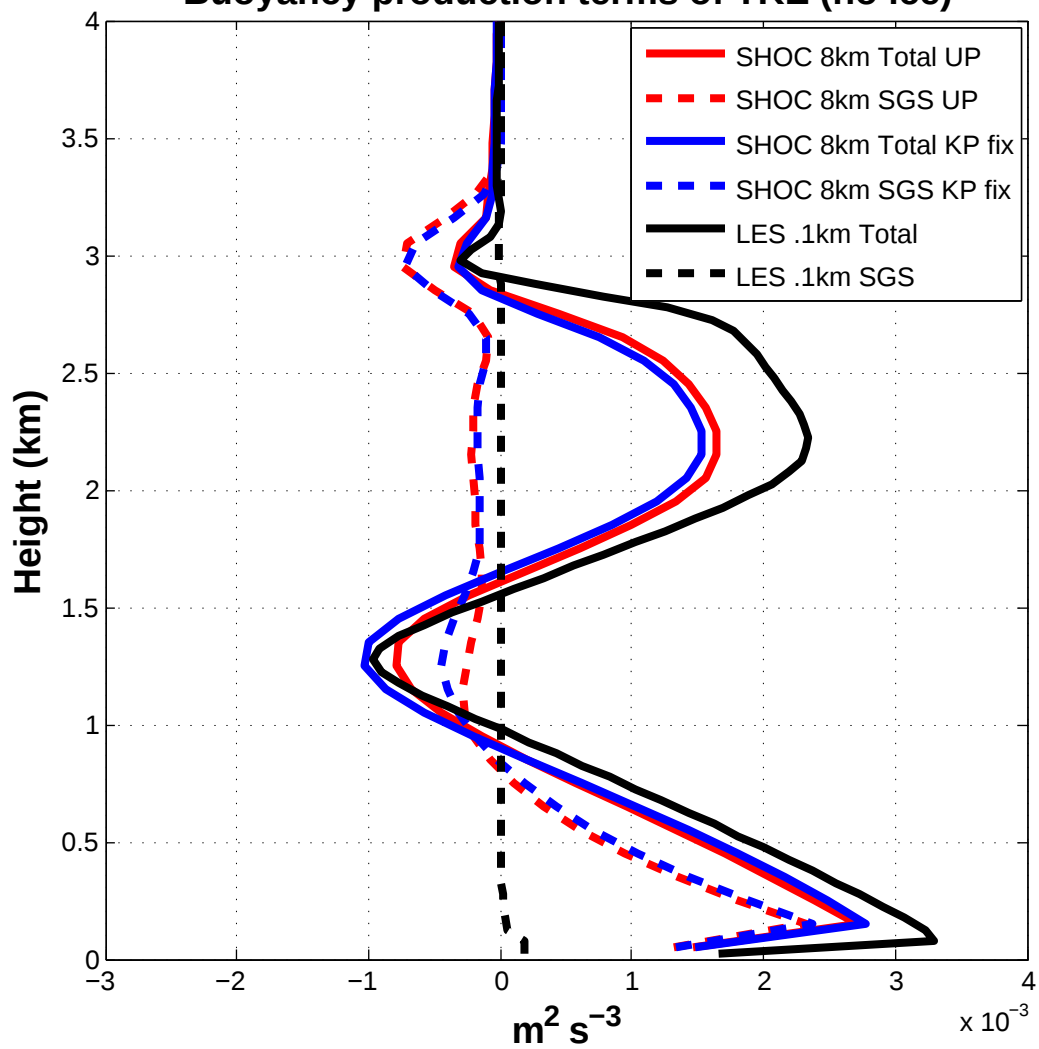
Buoyancy production terms of TKE (no ice)
