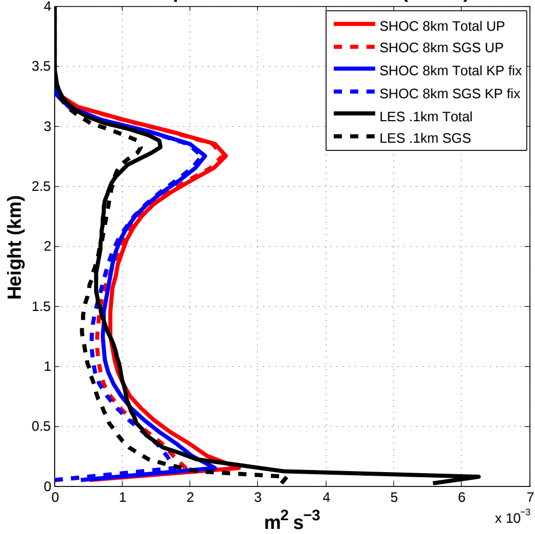
Shear production terms of TKE (no ice)
