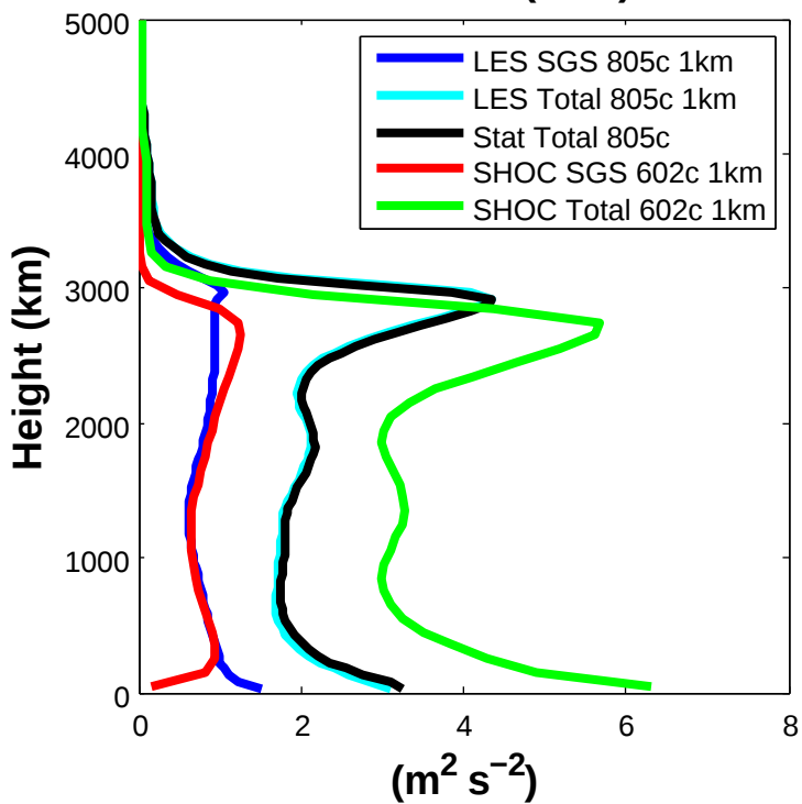
TKE No Ice (1km)
