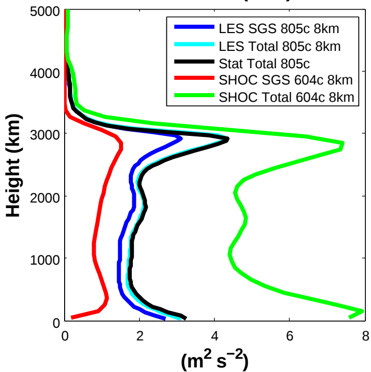
TKE No Ice (8km)
