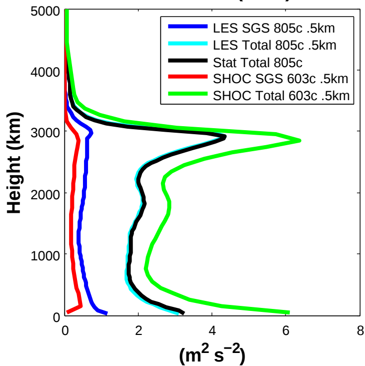
TKE No Ice (.5km)
