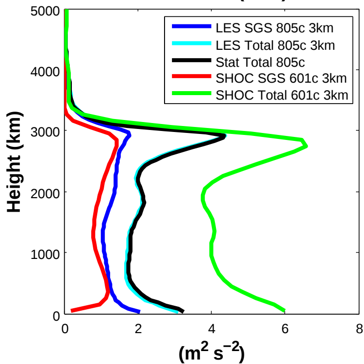
TKE No Ice (3km)
