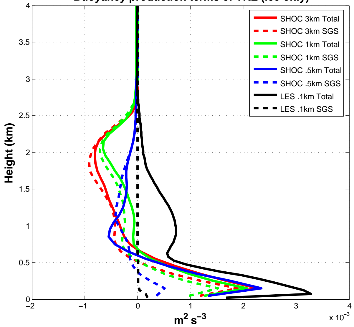
Buoyancy production terms of TKE (ice only)
