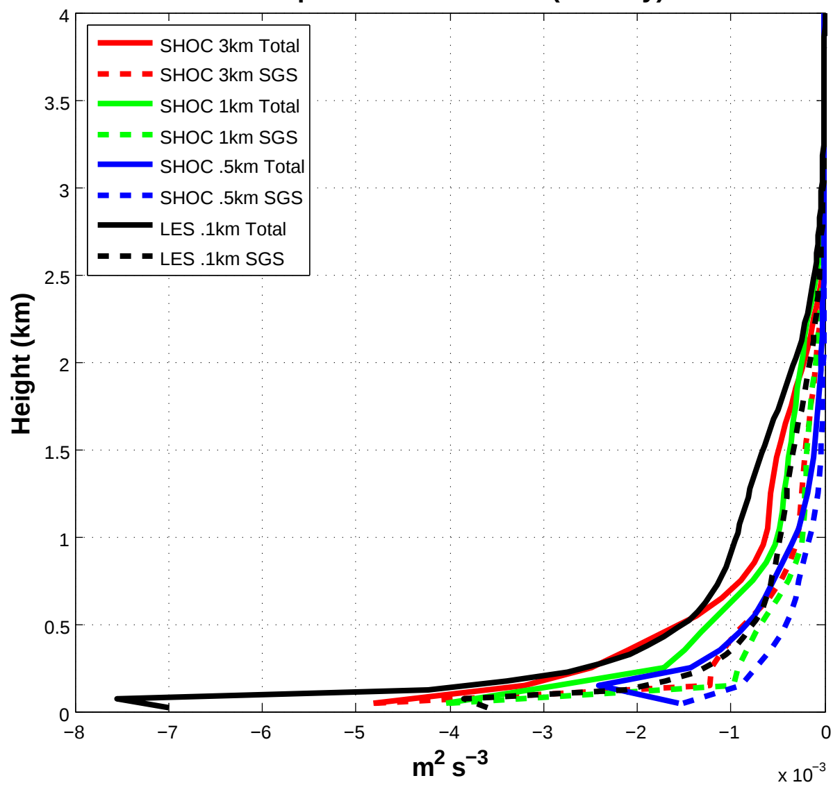
Dissipation terms of TKE (ice only)
