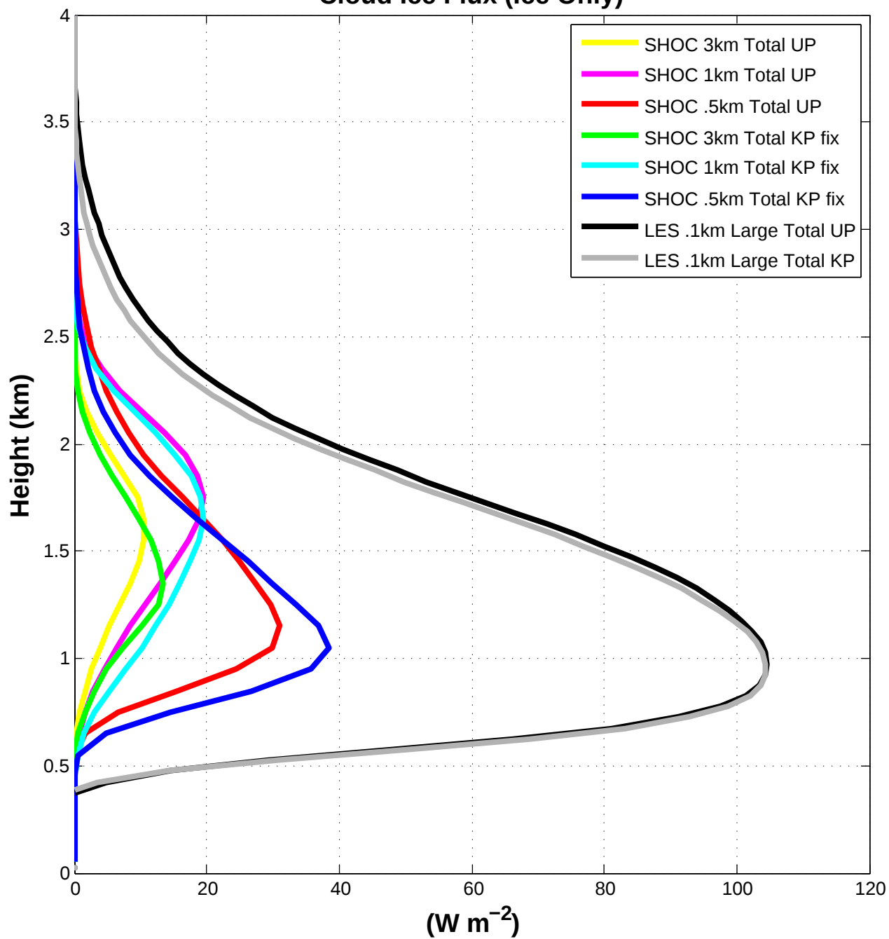
Cloud Ice Flux (Ice Only)
