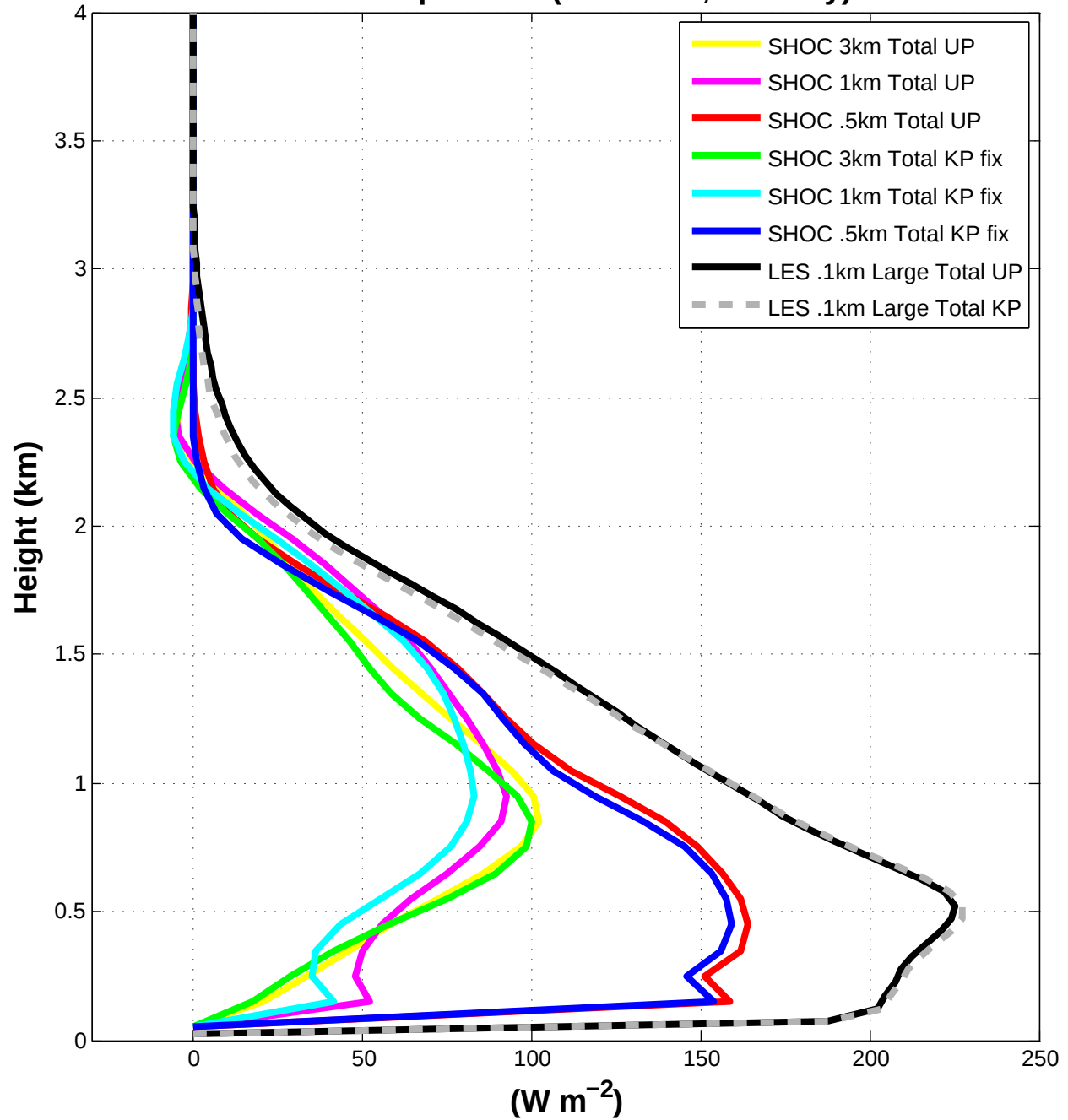
Water Vapor Flux (Resolved, Ice Only)
