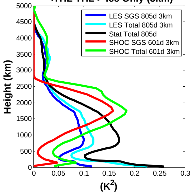
<THL'THL'> Ice Only (3km)
