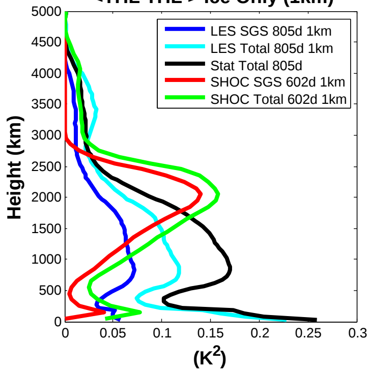
<THL'THL'> Ice Only (1km)
