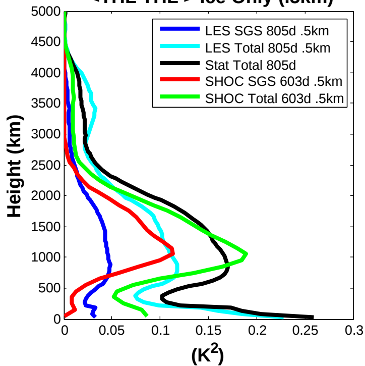
<THL'THL'> Ice Only (.5km)
